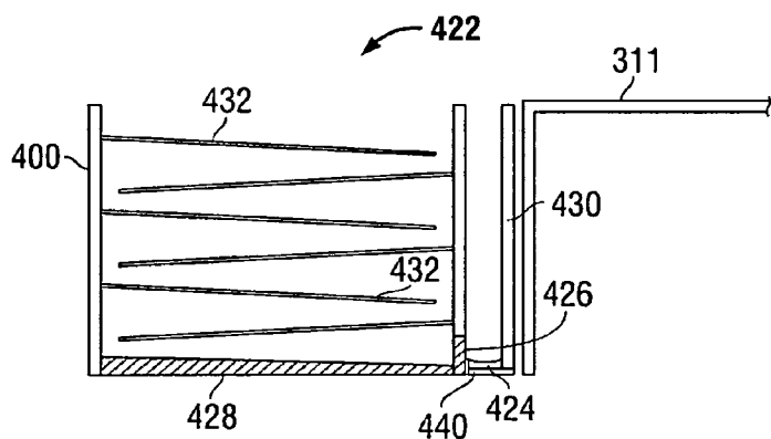
FIG. 23D
