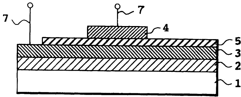
FIG. 1 (PRIOR ART)
