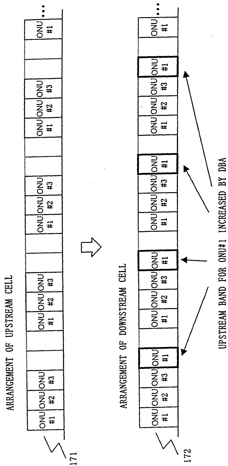
Fig. 8 RELATED ART
