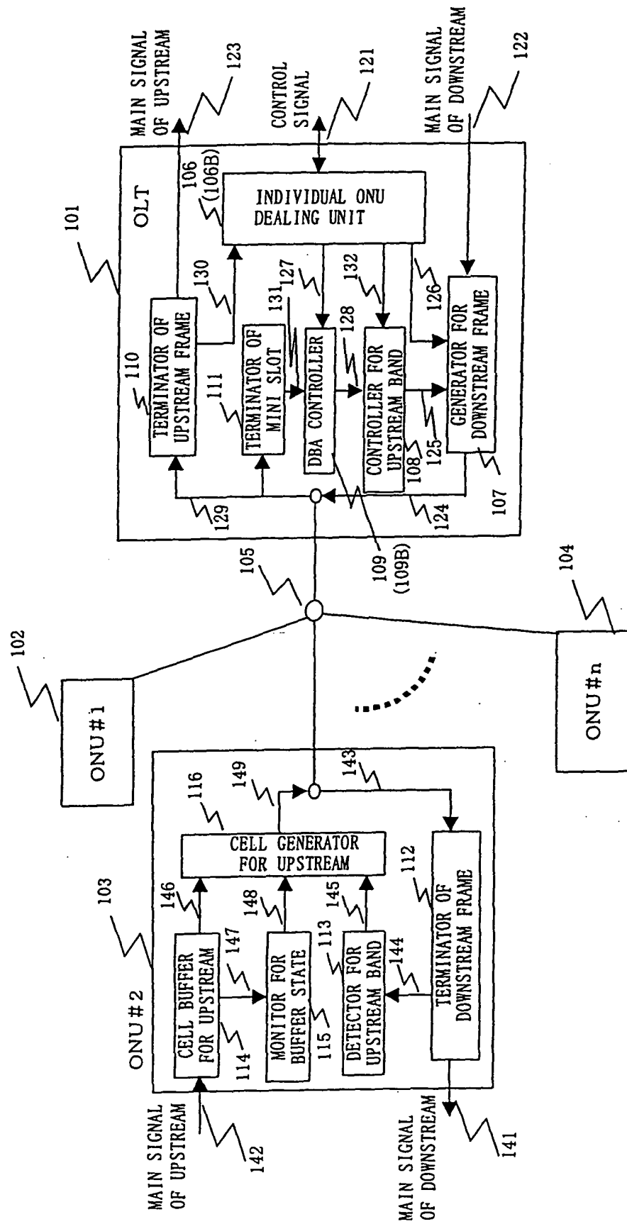
Fig. 3 RELATED ART
