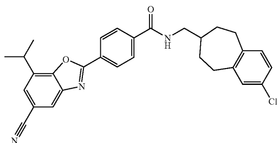
N-[(2-Chloro-6,7,8,9-tetrahydro-5H-benzo[7]annulen-7-yl)methyl]-4-(5-cyano-7-isopropyl-1,3-benzoxazol-2-yl)benzamide
