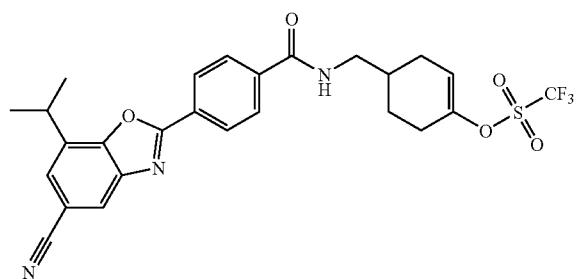
4-({[4-(5-Cyano-7-isopropyl-1,3-benzoxazol-2-yl)benzoyl]amino}methyl)cyclohex-1-en-1-yl trifluoromethanesulfonate
