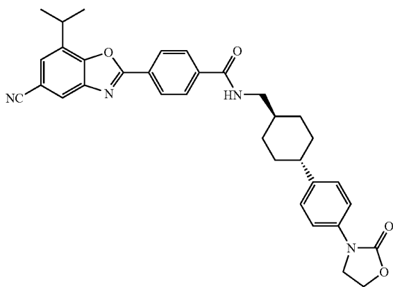
4-(5-cyano-7-isopropyl-1,3-benzoxazol-2-yl)-N- ({trans-4-[4-(2-oxo-1,3-oxazolidin-3-yl)phenyl] cyclohexyl}methyl)benzamide
