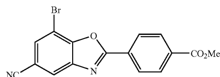
INTERMEDIATE 1
