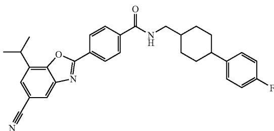
cis and trans 4-(5-Cyano-7-isopropyl-1,3-benzoxazol-2-yl)-N-([4-(4-fluorophenyl)cyclohexyl]methyl)benzamide
