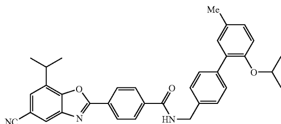
4-(5-cyano-7-isopropyl-1,3-benzoxazol-2-yl)-N-[(2'-isopropoxy-5'-methylbiphenyl-4-yl)methyl]benzamide
