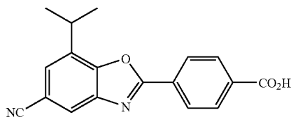
INTERMEDIATE 2
