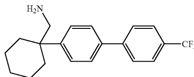
1-{1-[4'-(Trifluoromethyl)biphenyl-4-yl]cyclohexyl}methanamine
