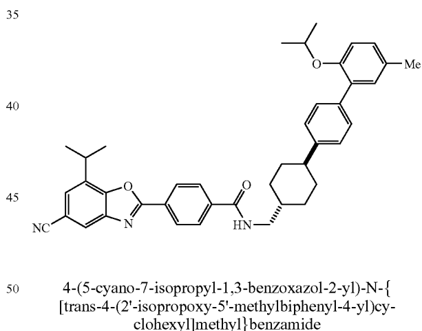
Example 87
