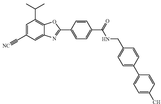
4-(5-Cyano-7-isopropyl-1,3-benzoxazol-2-yl)-N-[(4'-methylbiphenyl-4-yl)methyl]benzamide
