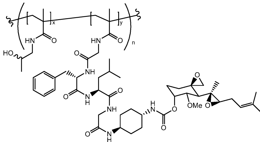
(Compound 1).
