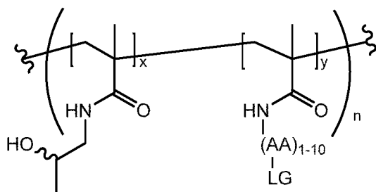
(Formula IV),
