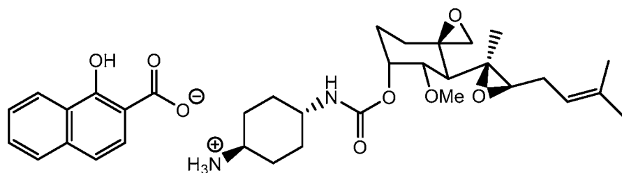
(Formula I);
