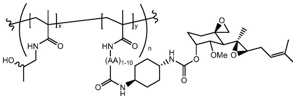
(Formula III).
