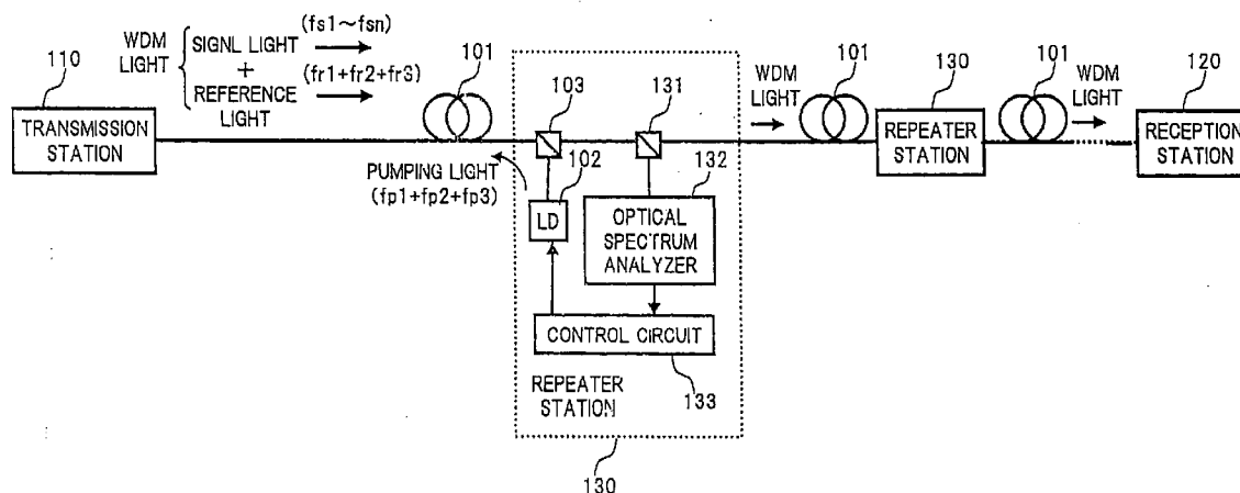
BLOCK DIAGRAM OF OPTICAL TRANSMISSION SYSTEM ACCORDING TO EMBODIMENT 1-1 OF PRESENT INVENTION
