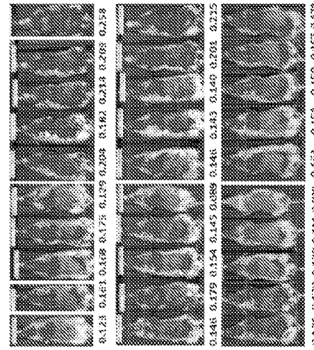
Anti-NME7 antibody 4A3 mouse vs humanized
