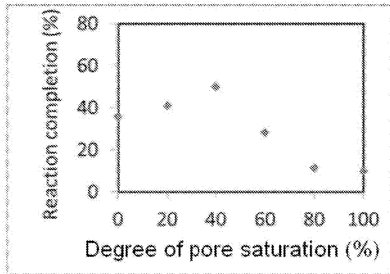
FIG. 10 (PRIOR ART)
