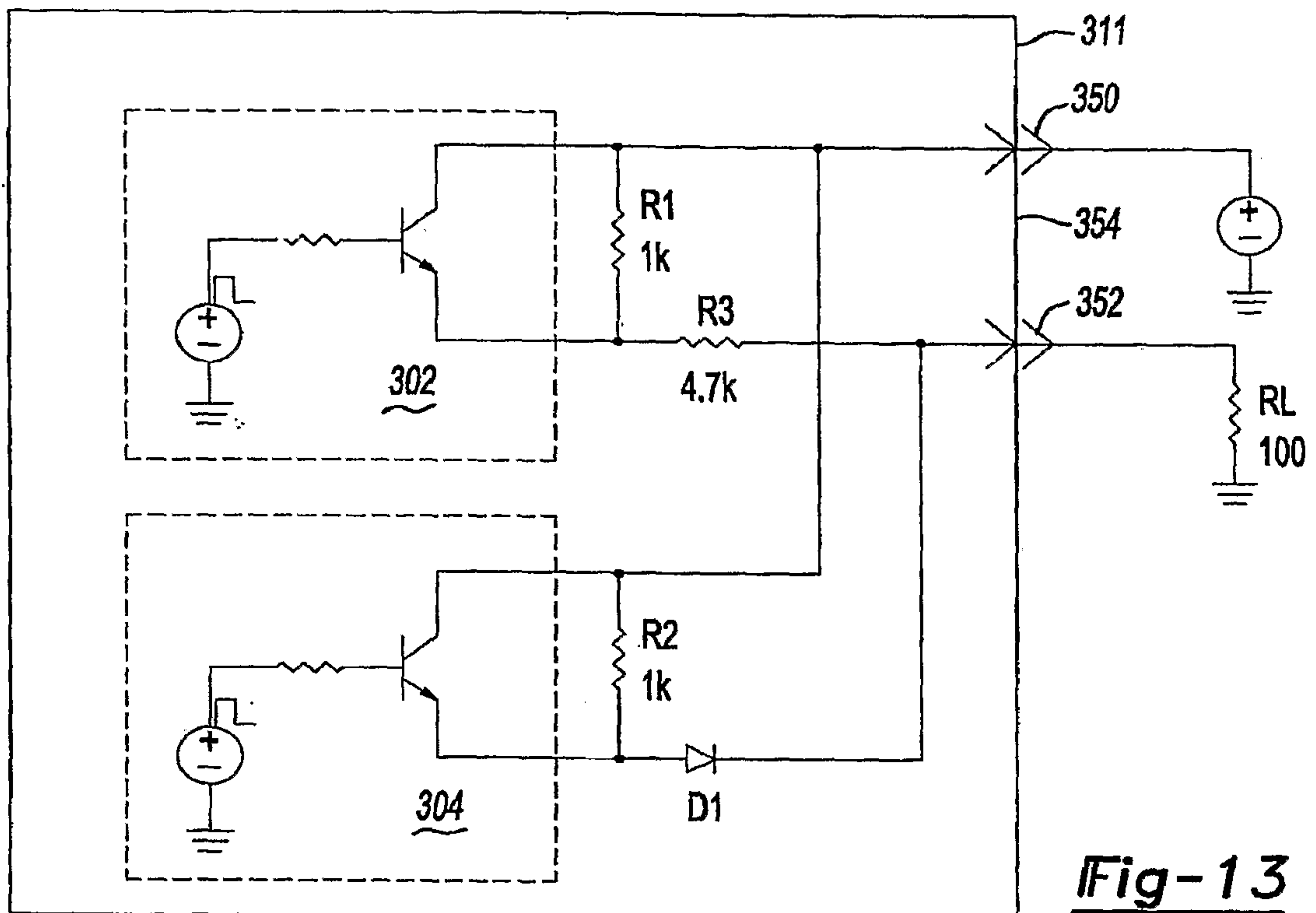
13/27 Sensor Configuration 1
