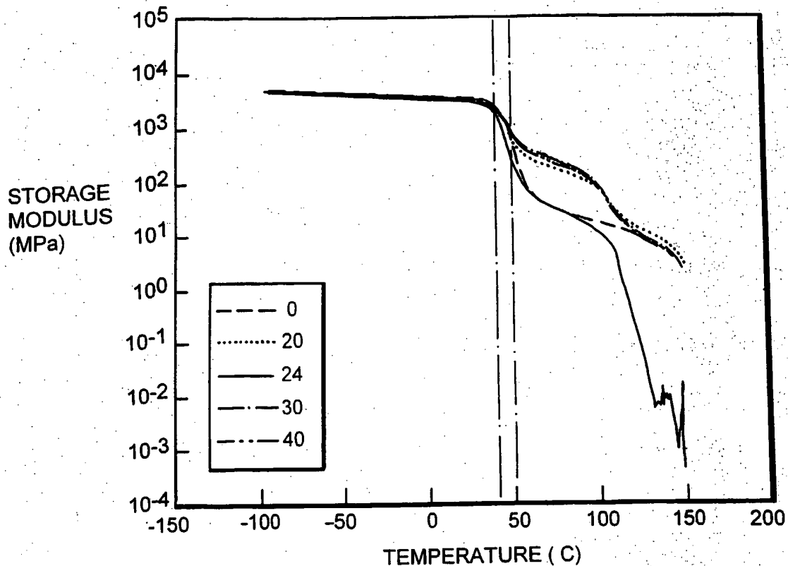
STORAGE MODULUS AS A FUNCTION OF PMMA CONTENT IN TERNARY BLENDS CONTAINING 70:30 PVAc/PVDF
