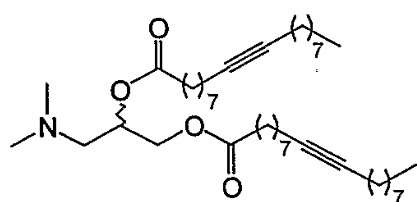
DH(9-yne)DAP (45)
