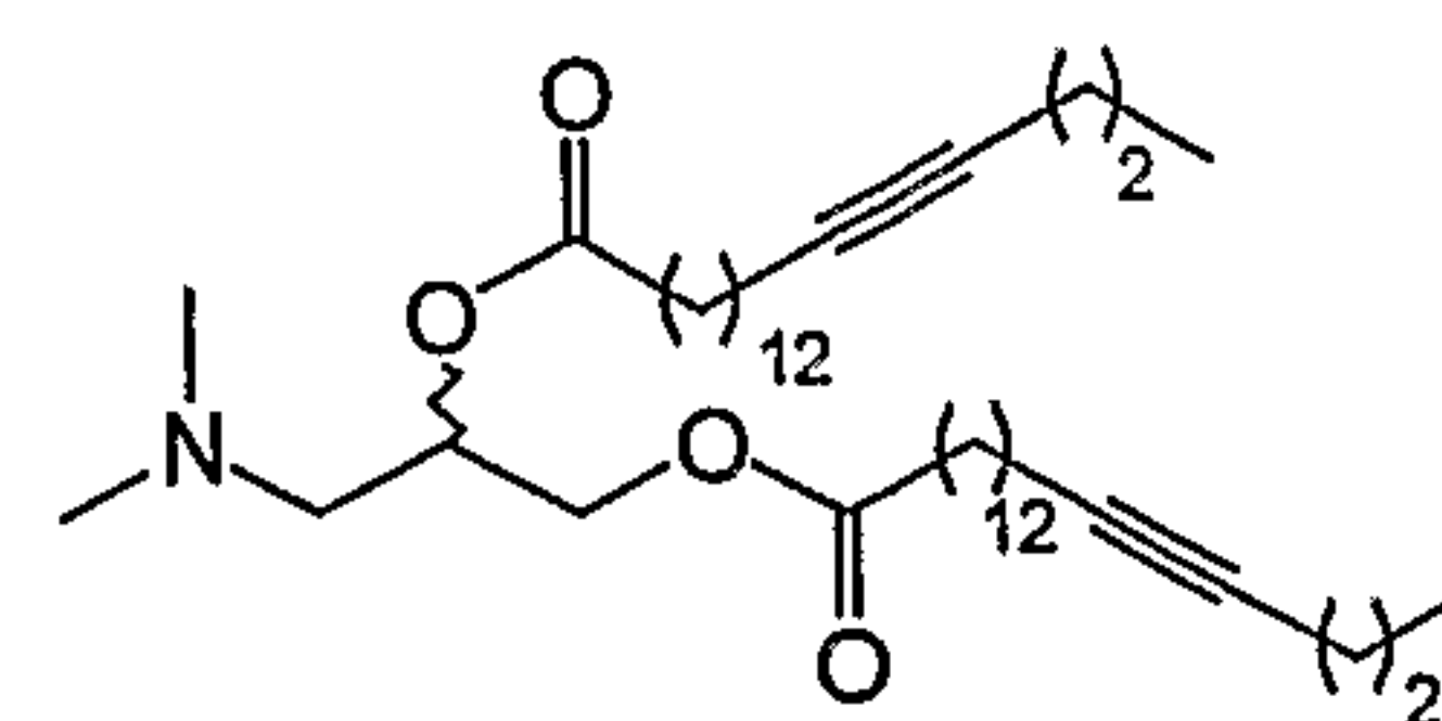
DO(14-yne)DAP (44)
