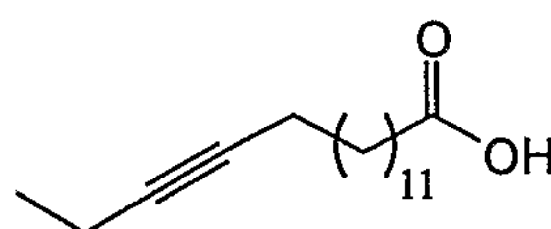
Heptadeca-14-ynoic Acid (9)
