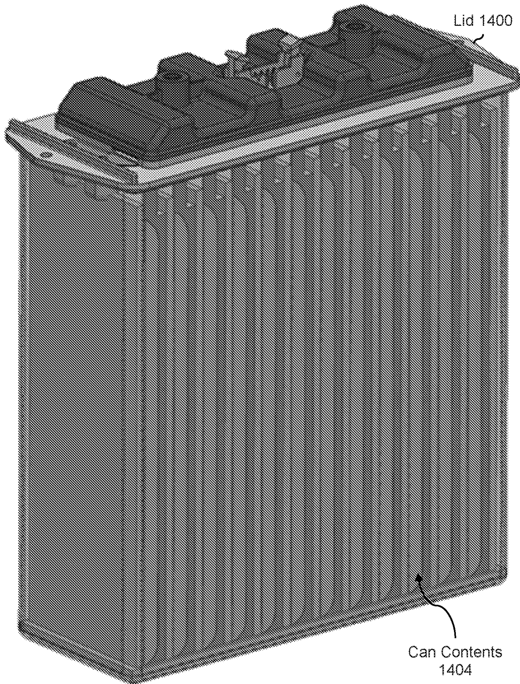
Side View (Cutaway)
