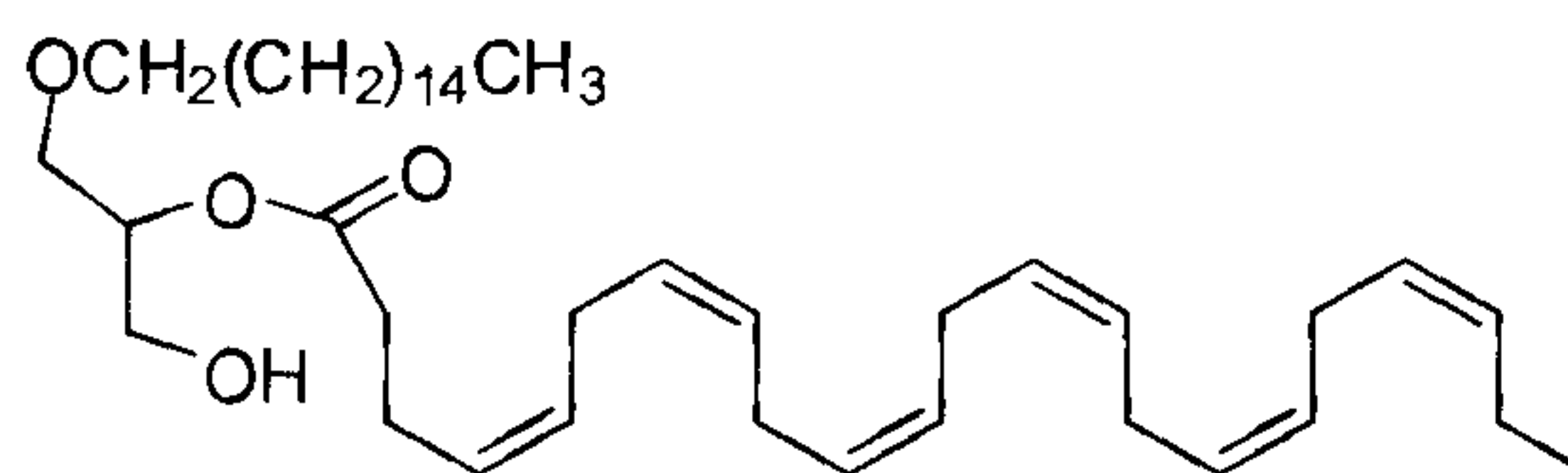
(4Z,7Z,10Z,13Z,16Z,19Z)-1-(hexadecyloxy)-3-hydroxypropan-2-yl docosa-4,7,10,13,16,19-hexaenoate
