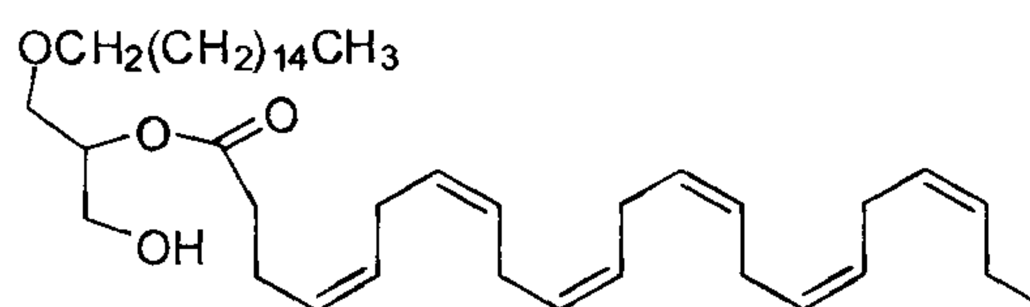
(4Z,7Z,10Z,13Z,16Z,19Z)-1-(hexadecyloxy)-3-hydroxypropan-2-yl docosa-4,7,10,13,16,19-hexaenoate
