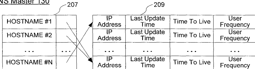
DNS Master 130
