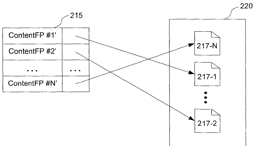
Object Archive 128
