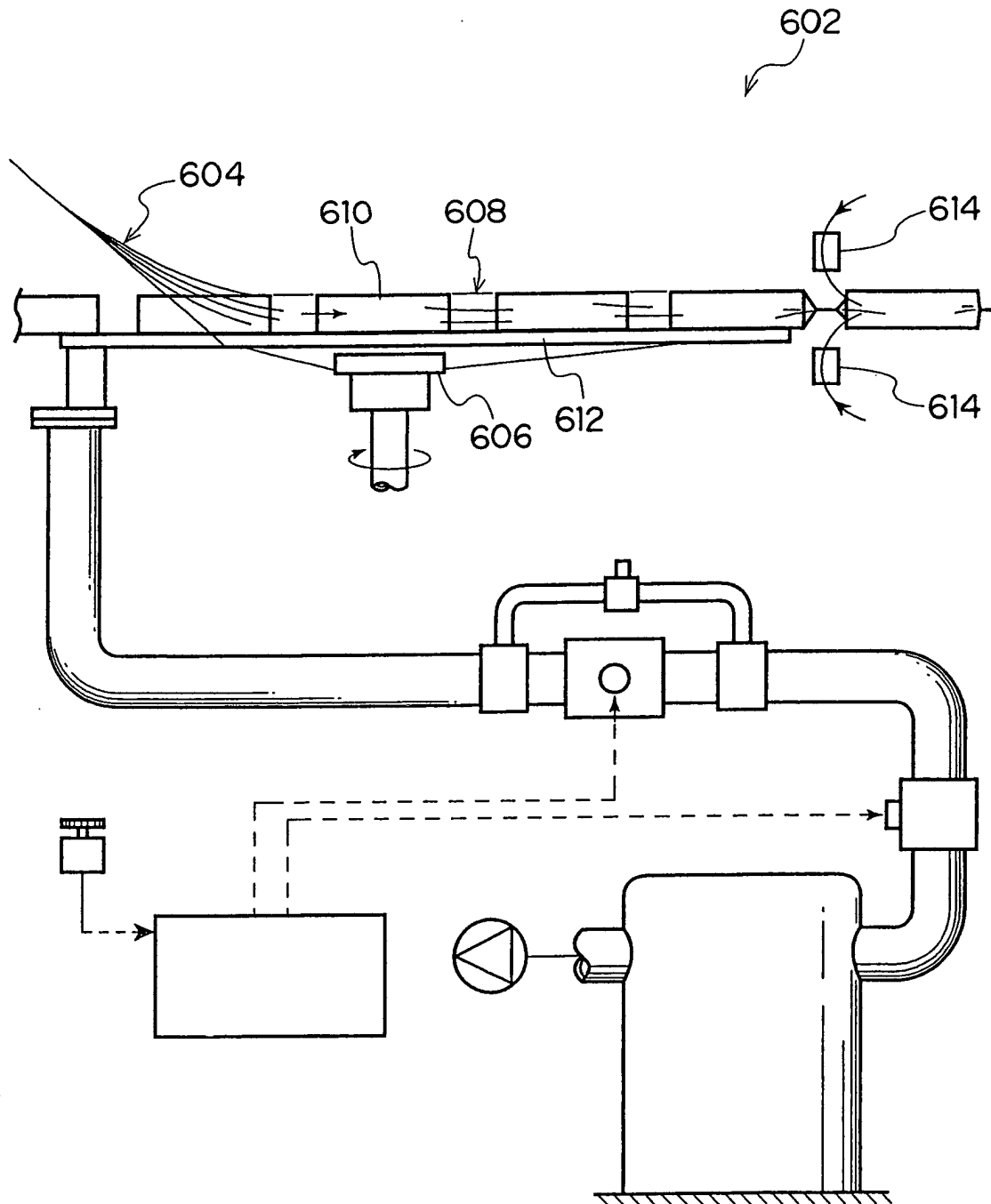
FIG.62 PRIOR ART
