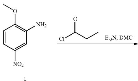
Scheme III
