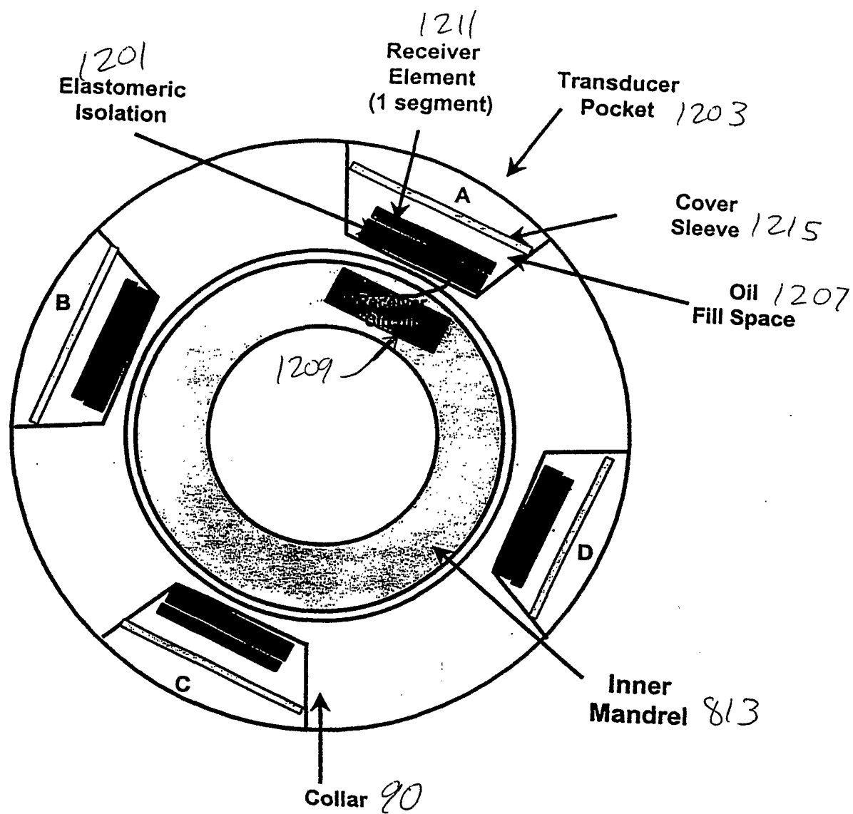
Figure 12 Individual Segmented Receiver Example
