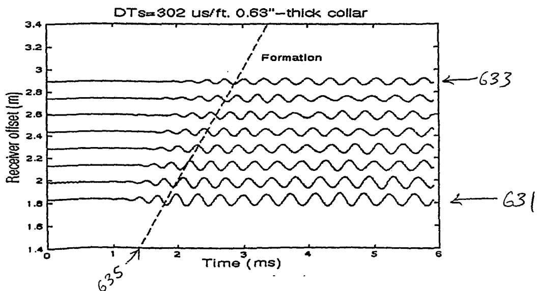
Figure 6B Quadrupole waveforms, thin collar pipe
