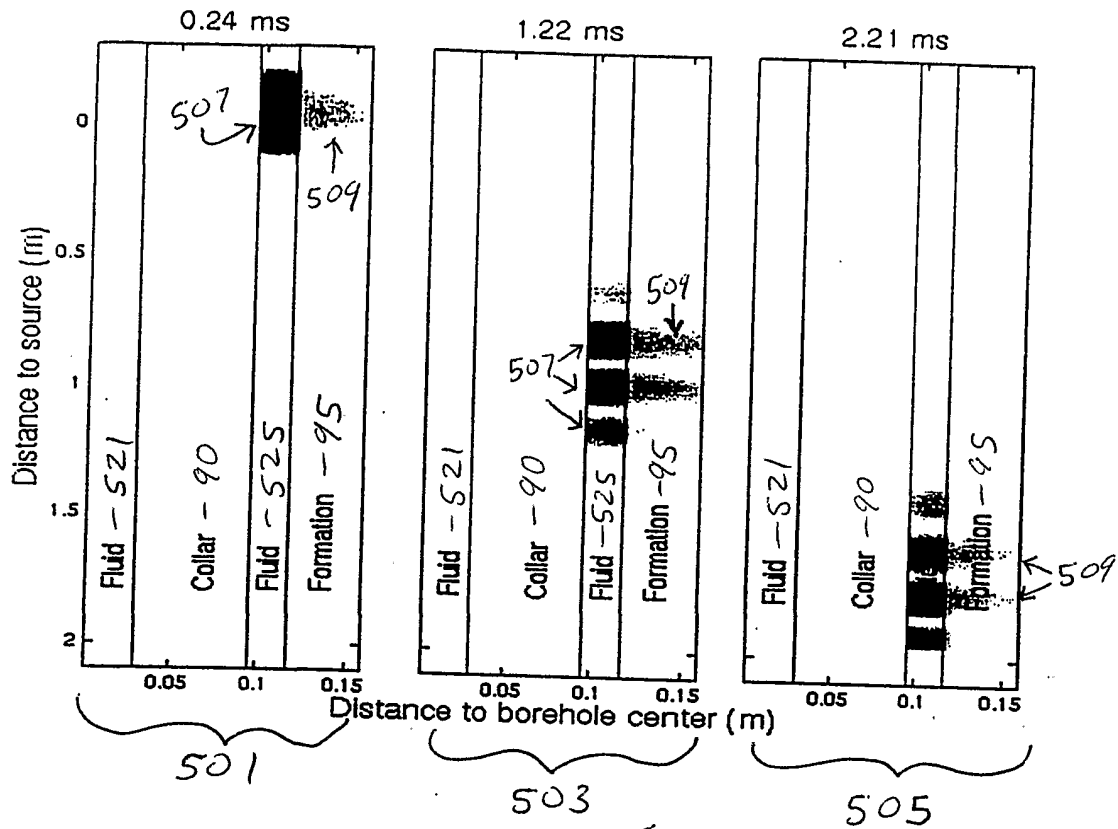
Figure 5A Wavefield snapshots
