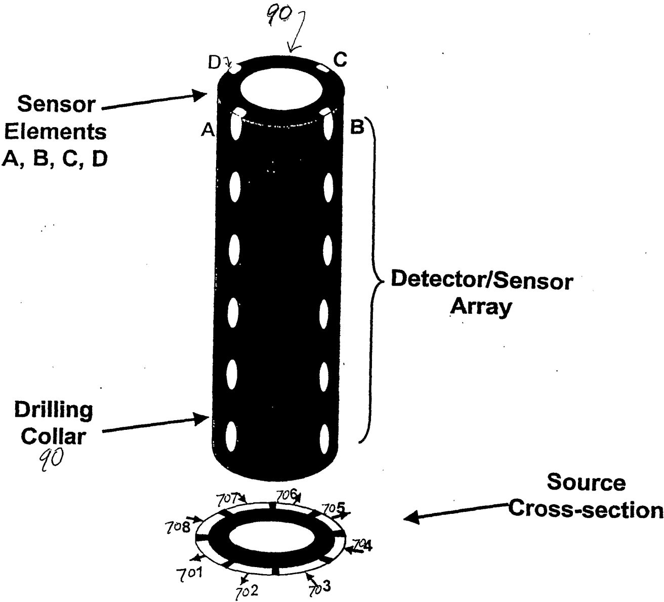
Figure 10 Sensor Array Layout
