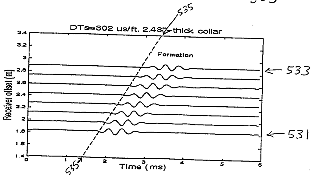
Figure 5B Quadrupole waveforms at various offsets
