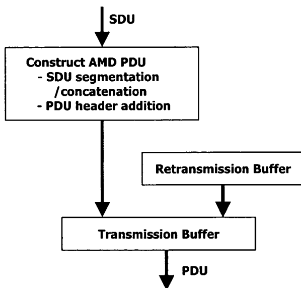
FIG.5 BACKGROUND ART
