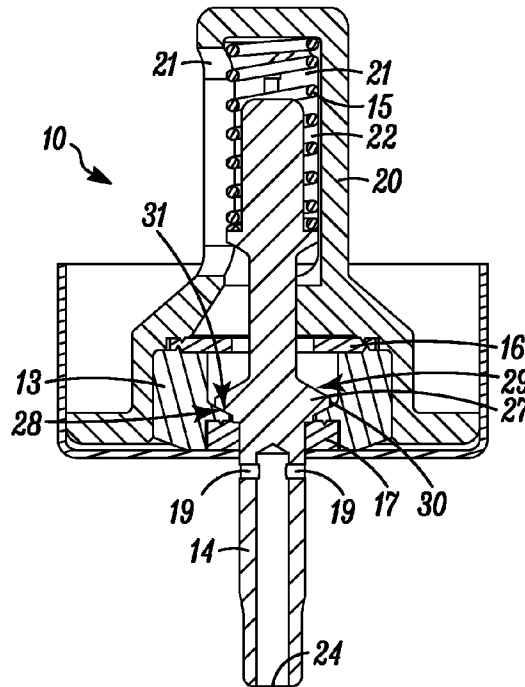
FIG. 3 Prior Art
