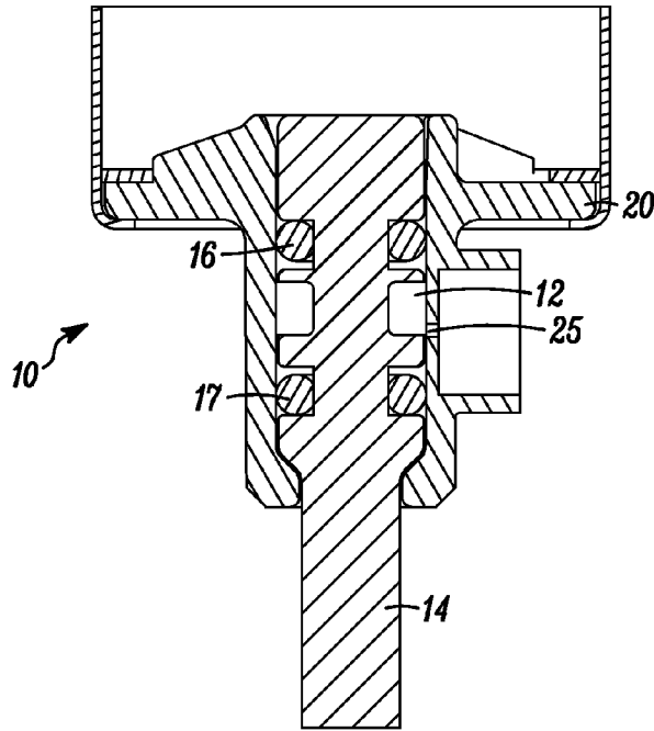
FIG. 2 Prior Art
