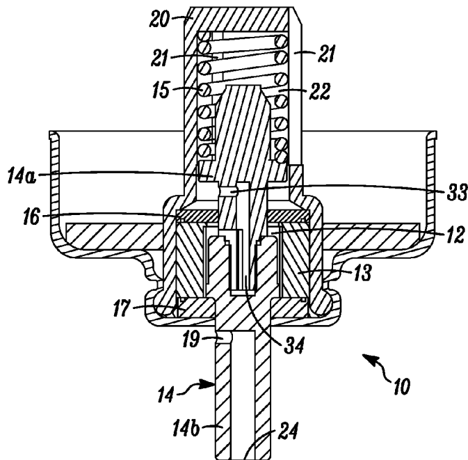
FIG. 5 Prior Art
