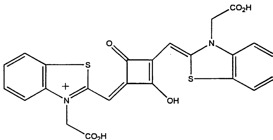
Benzothiazolium Squaraine Dye
