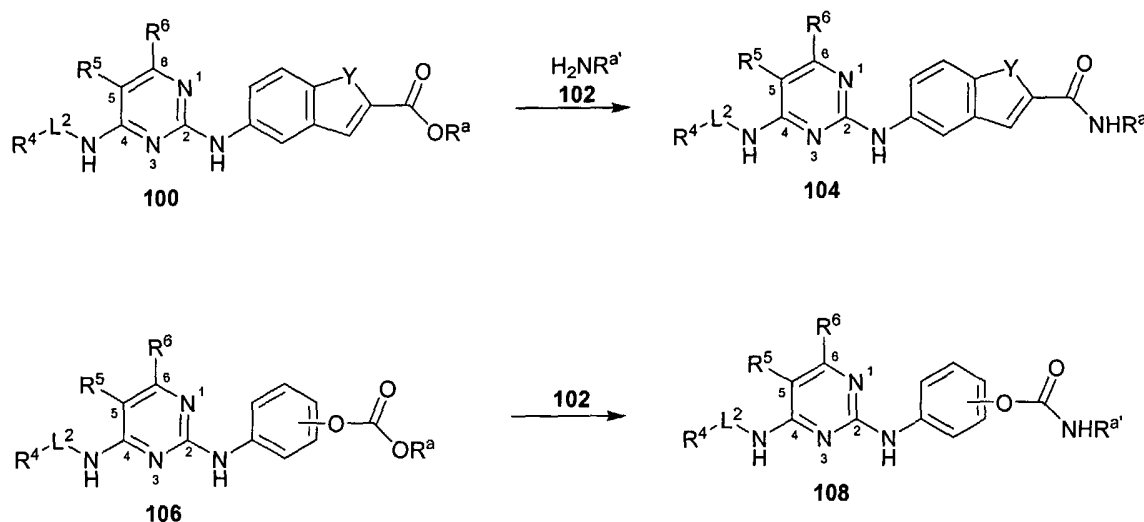
Scheme (X)
