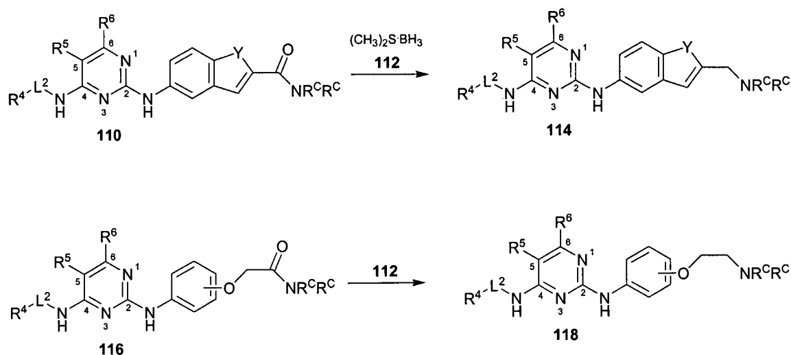
Scheme (XI)
