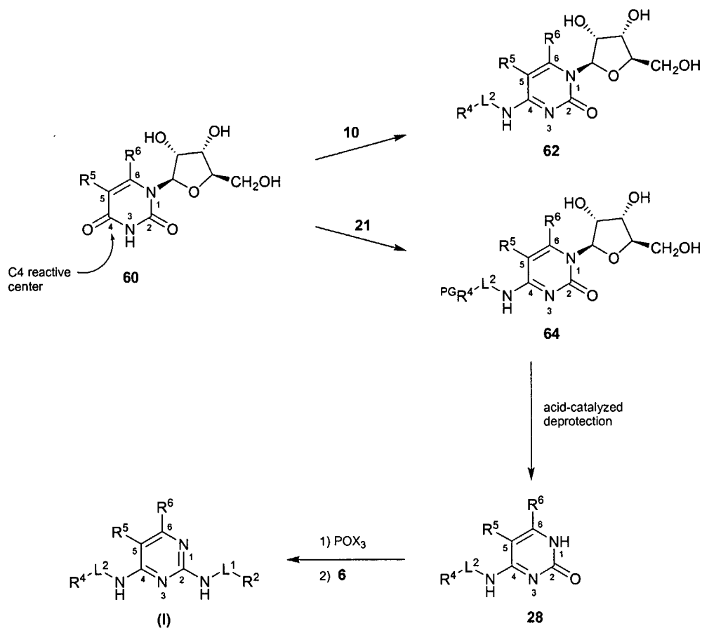
Scheme (VI)
