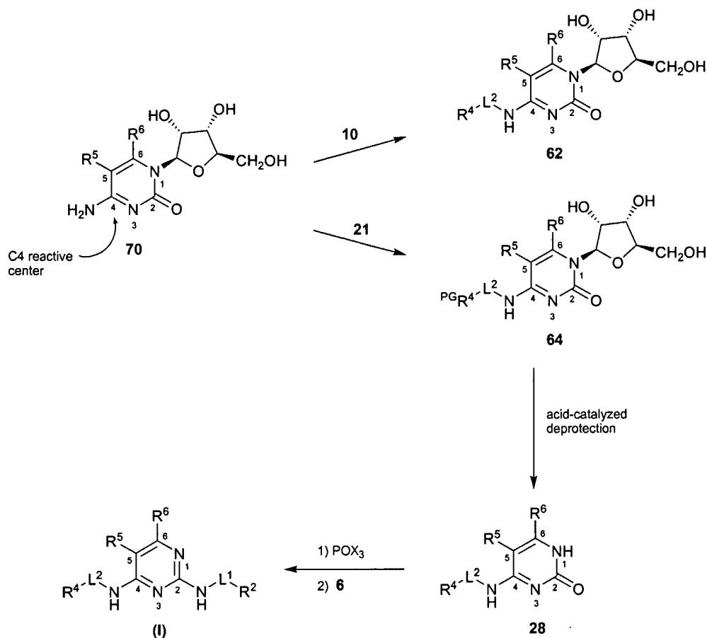
Scheme (VII)
