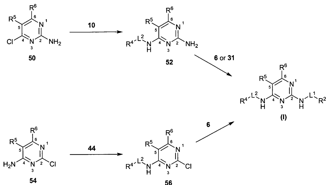
Scheme (V)
