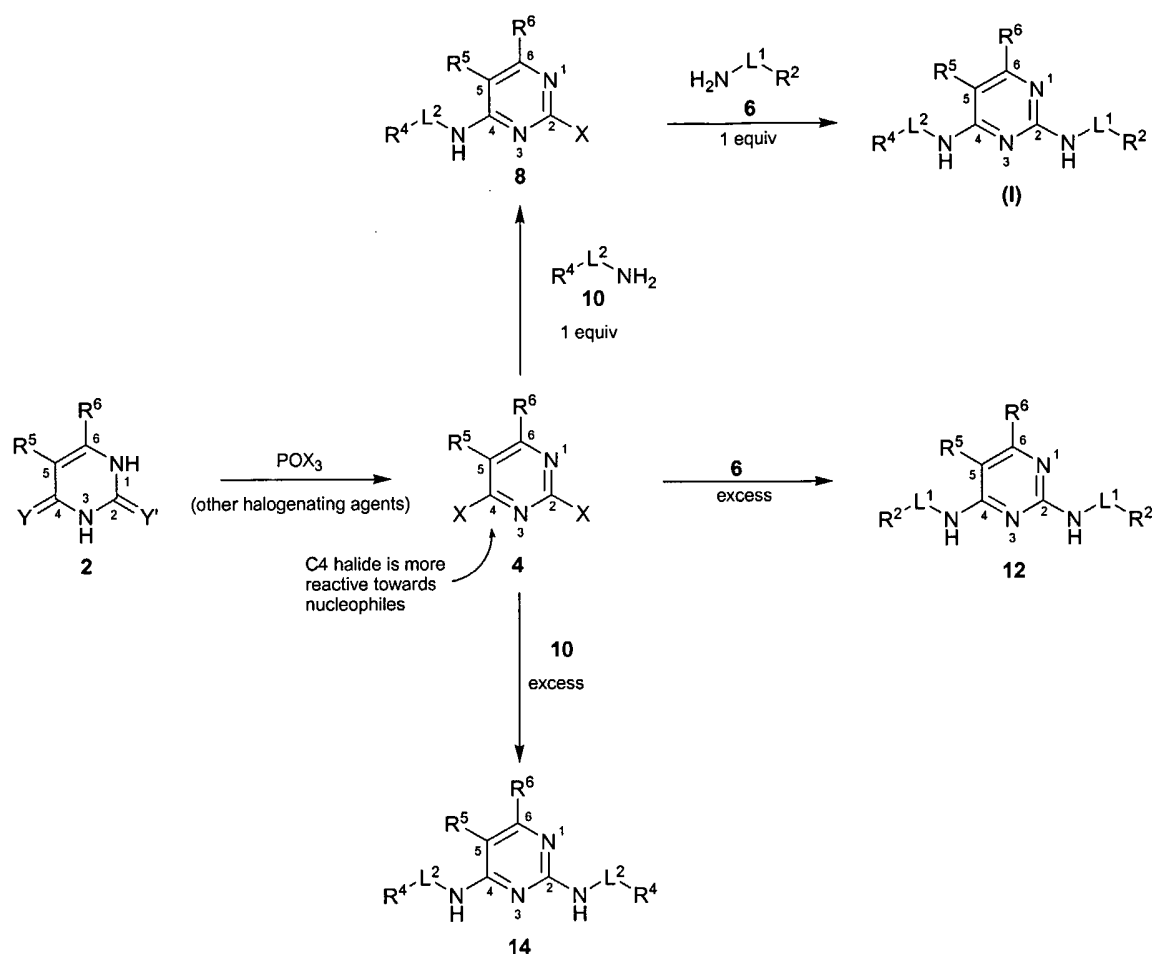
Scheme (I)
