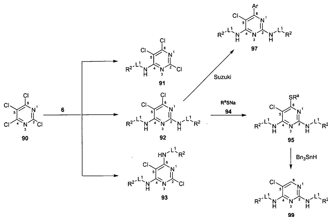
Scheme (IX)
