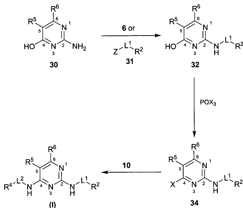
Scheme (III)
