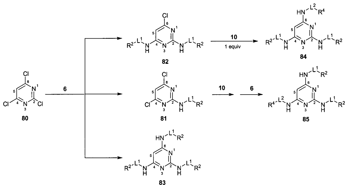
Scheme (VIII)
