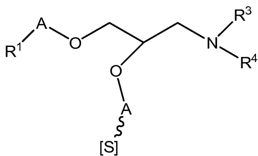
Formula IVa
