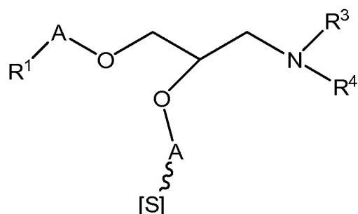
Formula IVa
