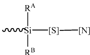
Formula IIC
