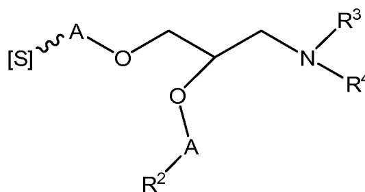
Formula IVb,
