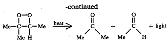
trimethyl-1,2-dioxetane
