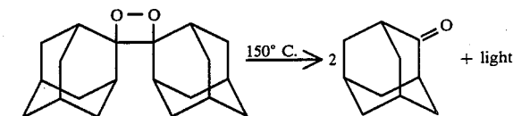
adamantylideneadamantane
