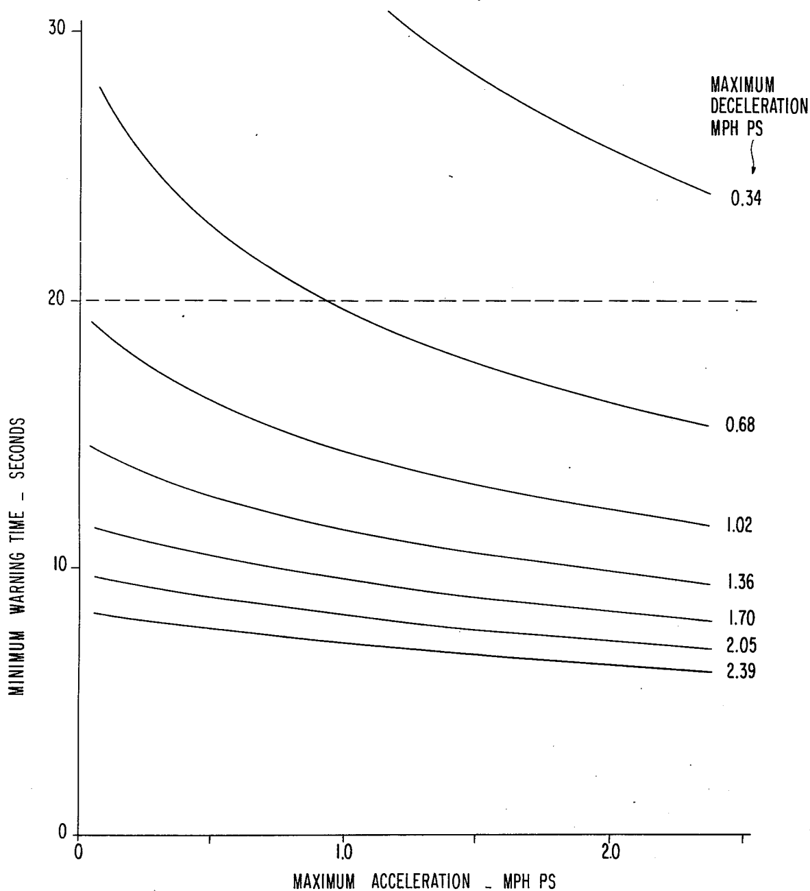
FIG. 16 MINIMUM WARNING TIME VERSUS MAXIMUM ACCELERATION FOR TRAINS WHICH STAY ABOVE 20 MPH
