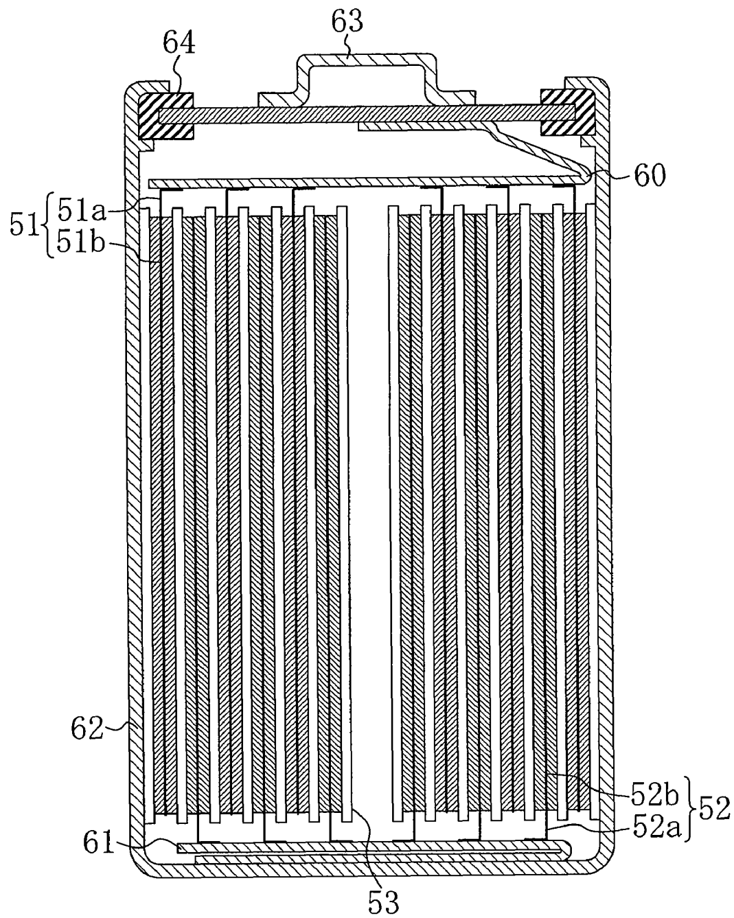
FIG. 17 PRIOR ART
