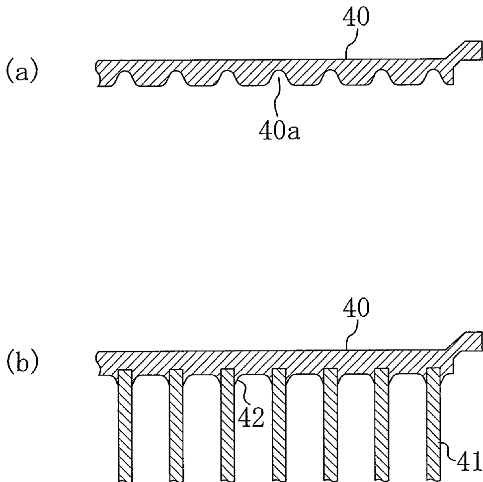
FIG. 16 PRIOR ART
