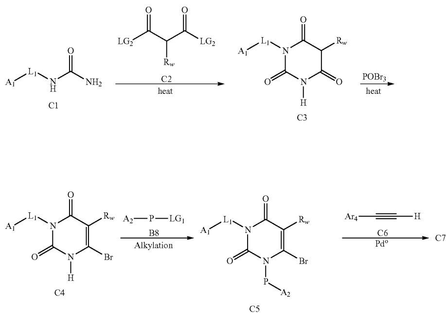
Scheme C
