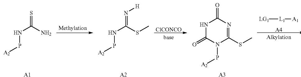
Scheme A
