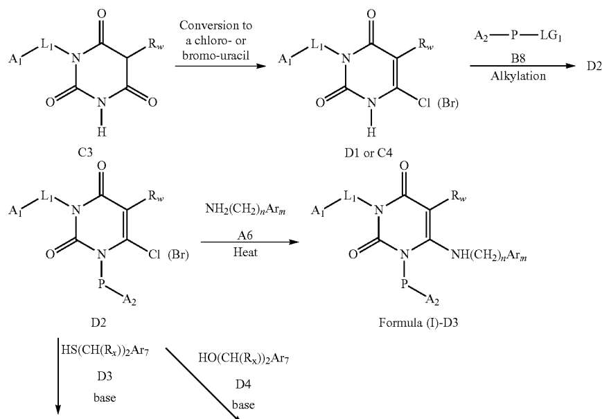
Scheme D
