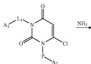
Scheme H
