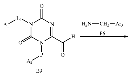
Scheme G
