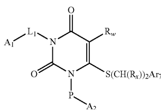
Formula (I)-D1
