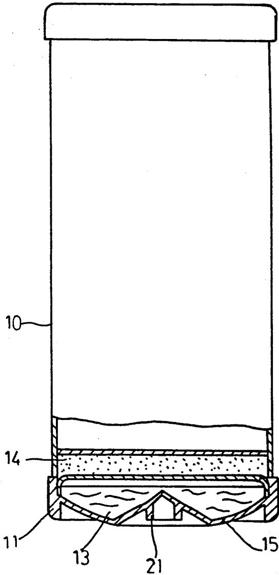
FIG. 2 (PRIOR ART)
