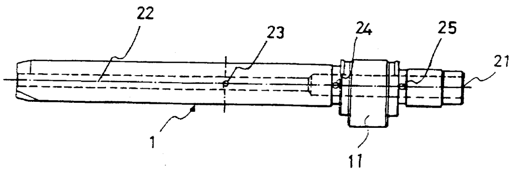
FIG. 3 CONVENTIONAL ART
