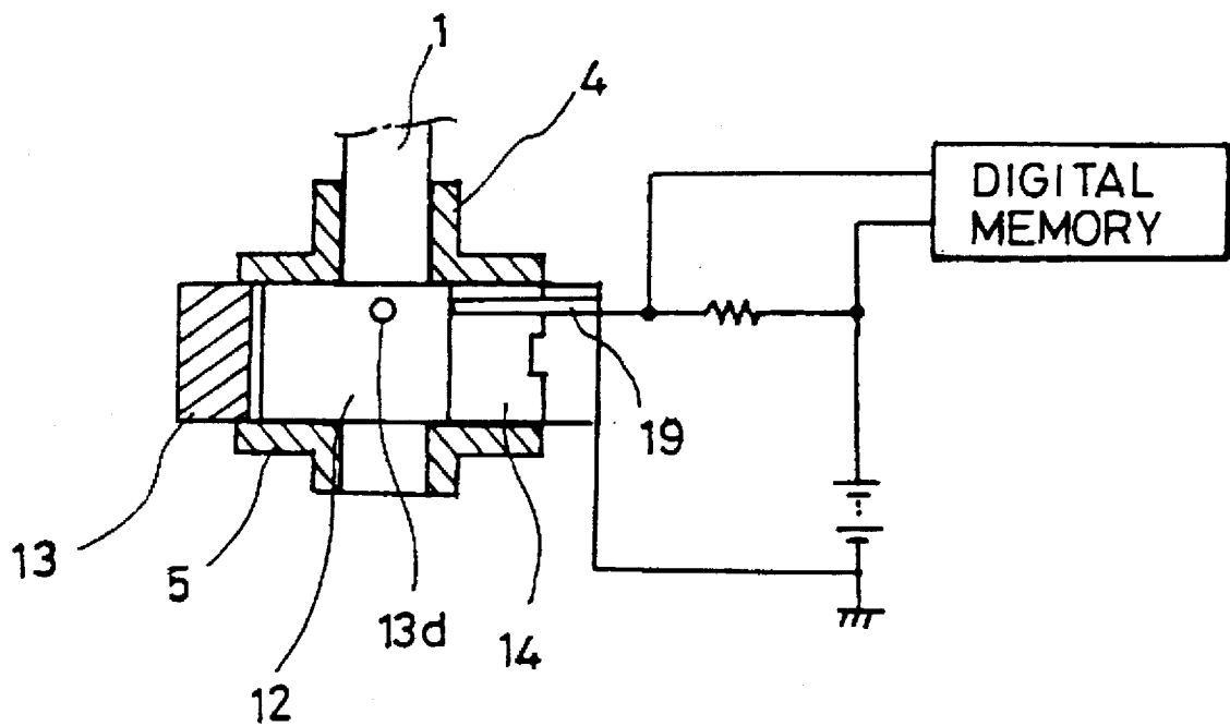
FIG. 6C CONVENTIONAL ART
