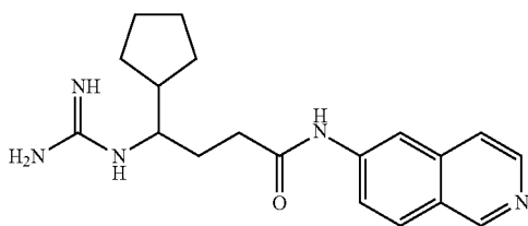
4-cyclopentyl-4-guanidino-N-(isoquinolin-6-yl)butanamide
