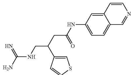
4-guanidino-N-(isoquinolin-6-yl)-3-(thiophen-3-yl)butanamide
