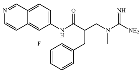
2-benzyl-N-(5-fluoroisoquinolin-6-yl)-3-(1-methylguanidino)propanamide
