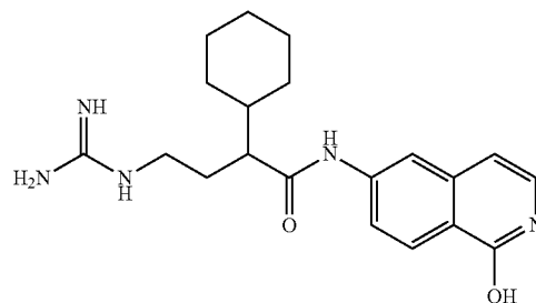
2-cyclohexyl-4-guanidino-N-(1-hydroxyisoquinolin-6-yl)butanamide
