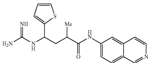
4-guanidino-N-(isoquinolin-6-yl)-2-methyl-4-(thiophen-2-yl)butanamide
