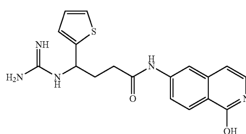
4-guanidino-N-(1-hydroxyisoquinolin-6-yl)-4-(thiophen-2-yl)butanamide
