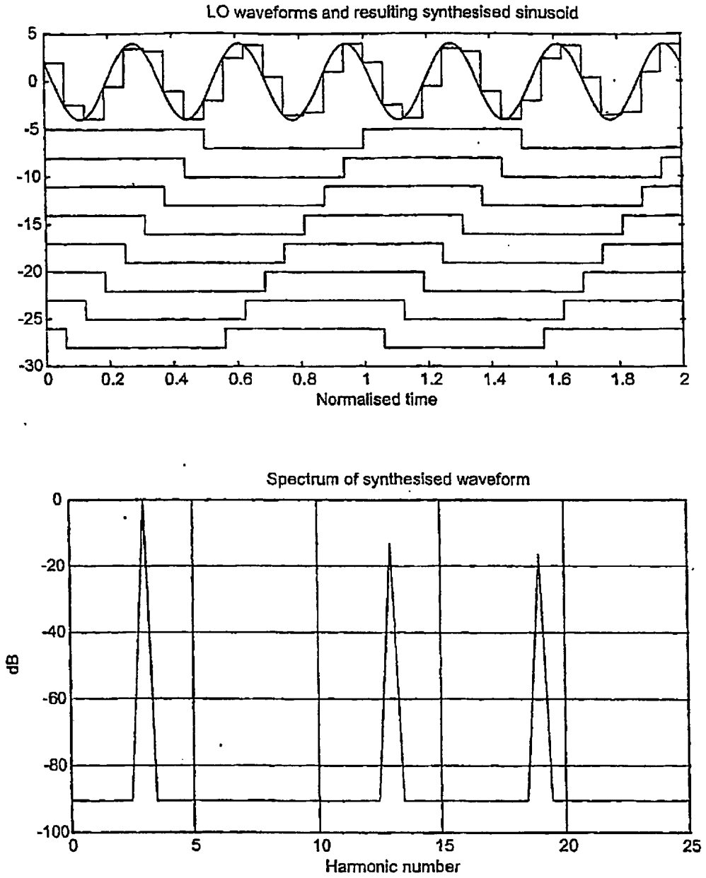
FIG. 7 8 phase, 3 cycle, 1 LO
