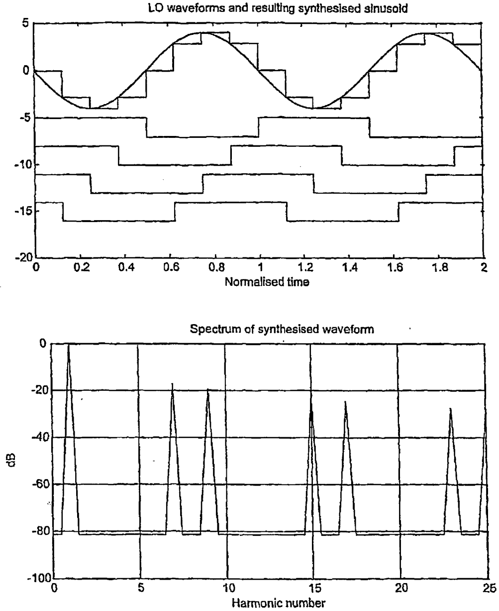
FIG. 9 4 phase, 1 cycle, I LO
