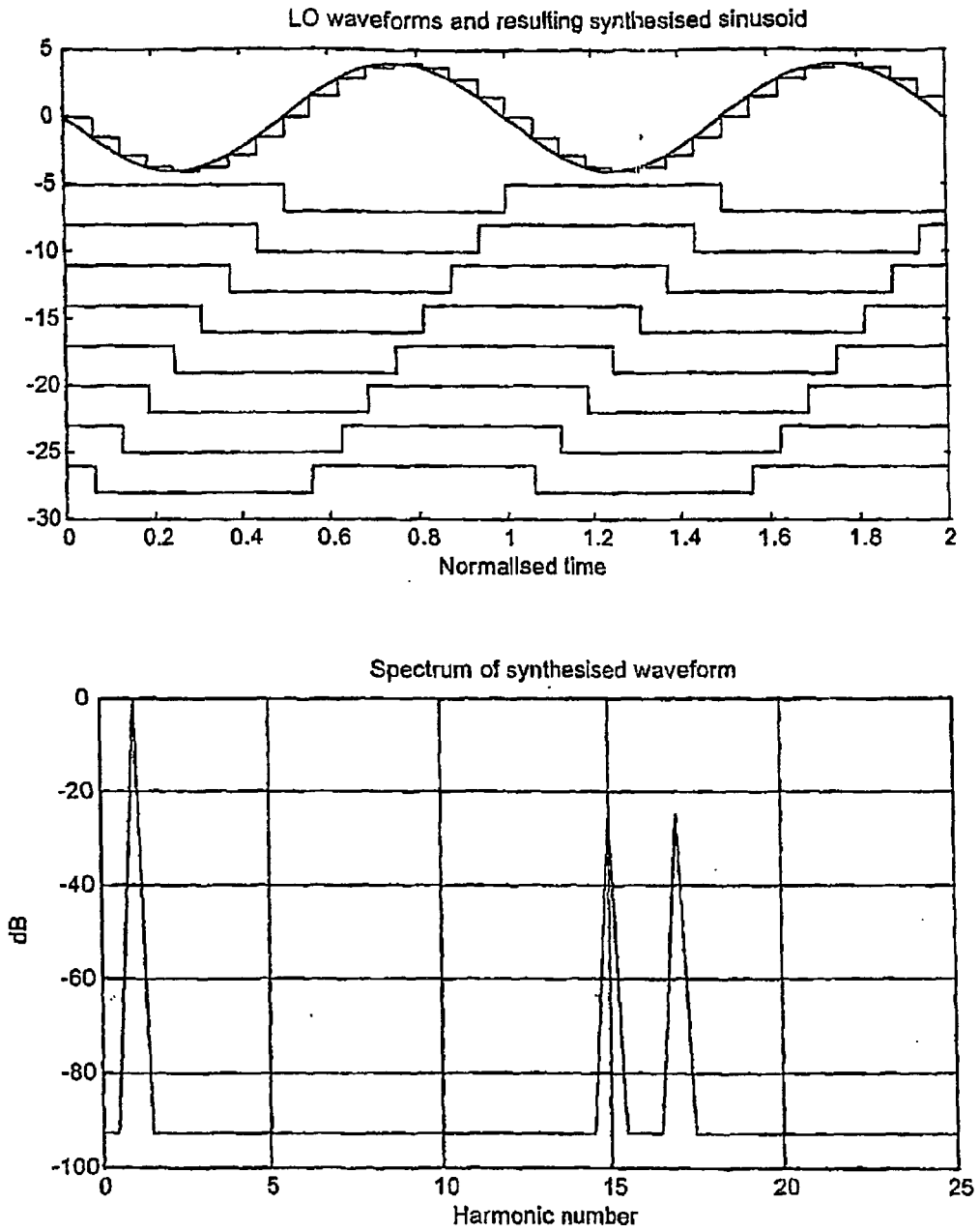
FIG. 5 8 phase, 1 cycle, I LO
