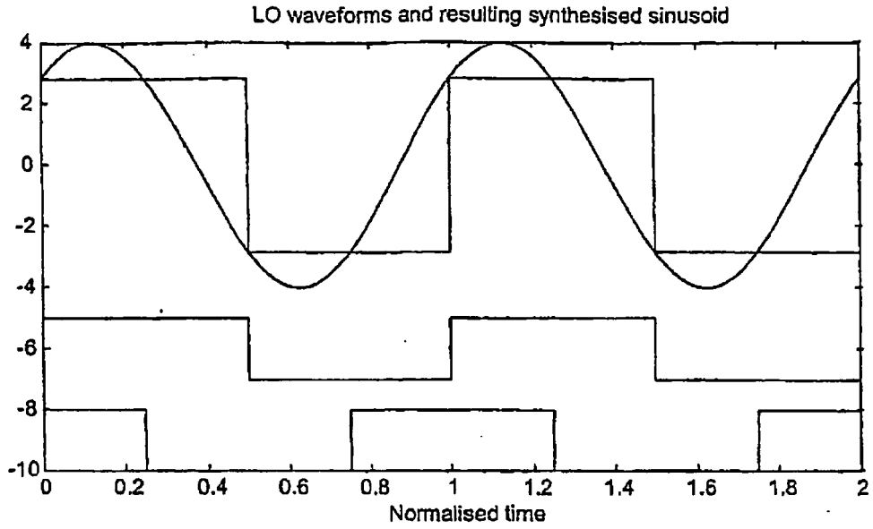
FIG. 12 2 phase, 1 cycle, Q LO
