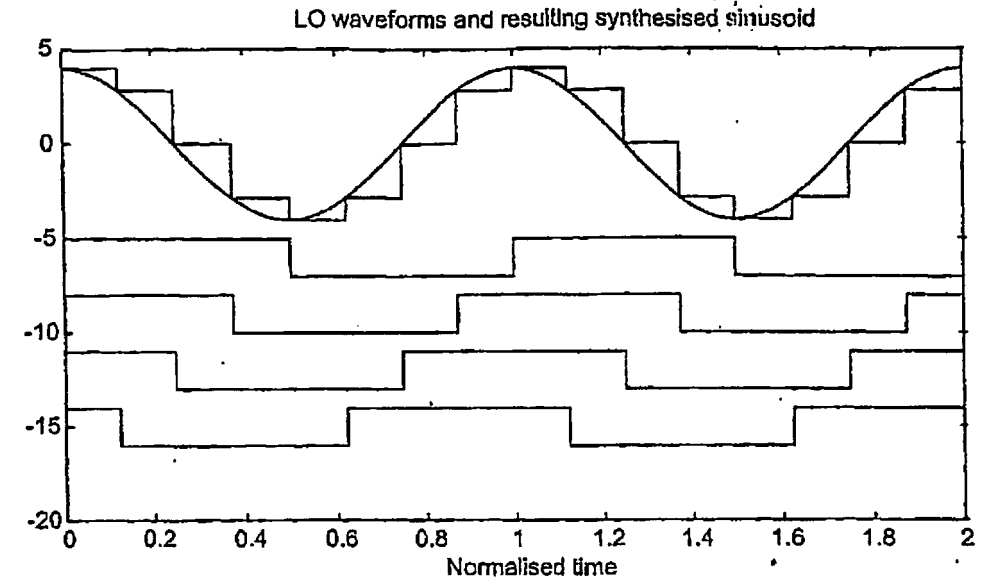
FIG. 10 4 phase, 1 cycle, Q LO
