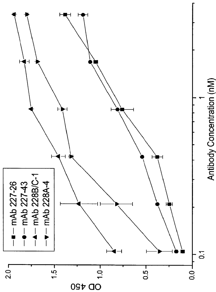
Fig. 2 Binding of anti-IL13 mAbs to MT-IL13/Fc
