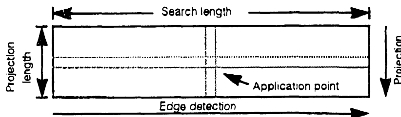
Figure 107. The Caliper Tool window
