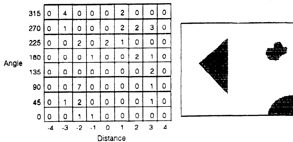
Figure 88. The final Hough space and the input image
