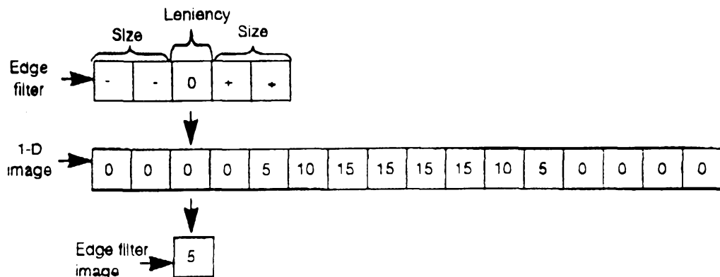
Figure 114. The edge filter is positioned in the one-dimensional image.
