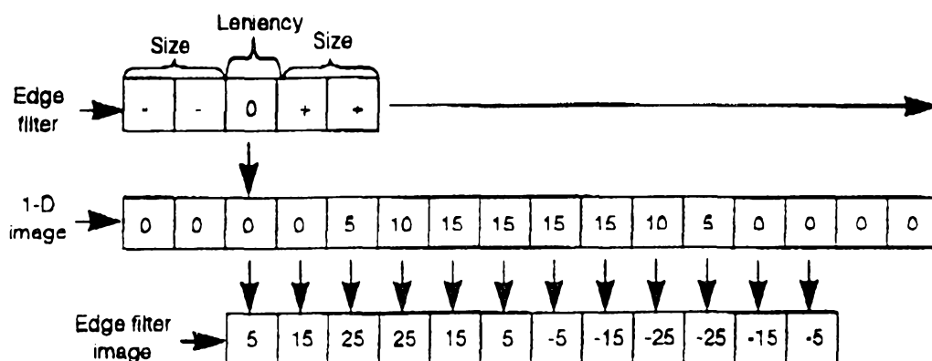
Figure 115. The edge filter is applied at each successive pixel until the edge filter no longer fits entirely in the image.
