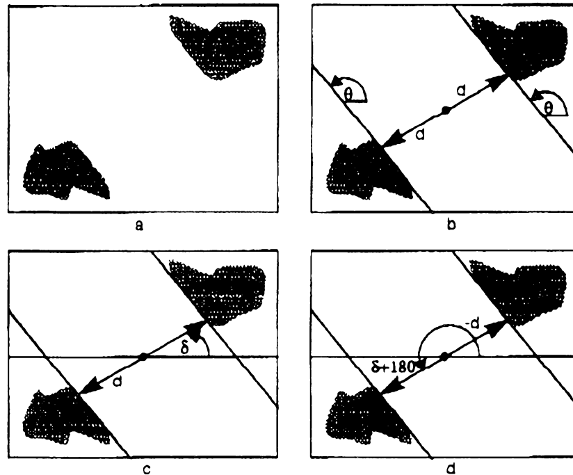
Figure 82. The angle of the distance vector determines the sign of the distance
