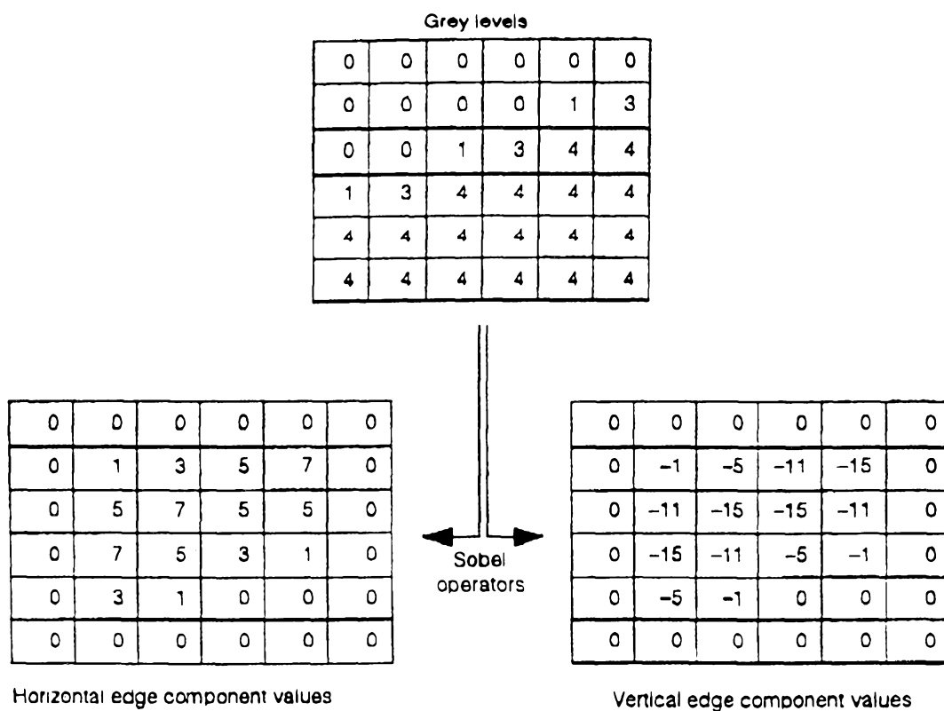
Figure 74. Horizontal and vertical edge component values computed with the Sobel operators
