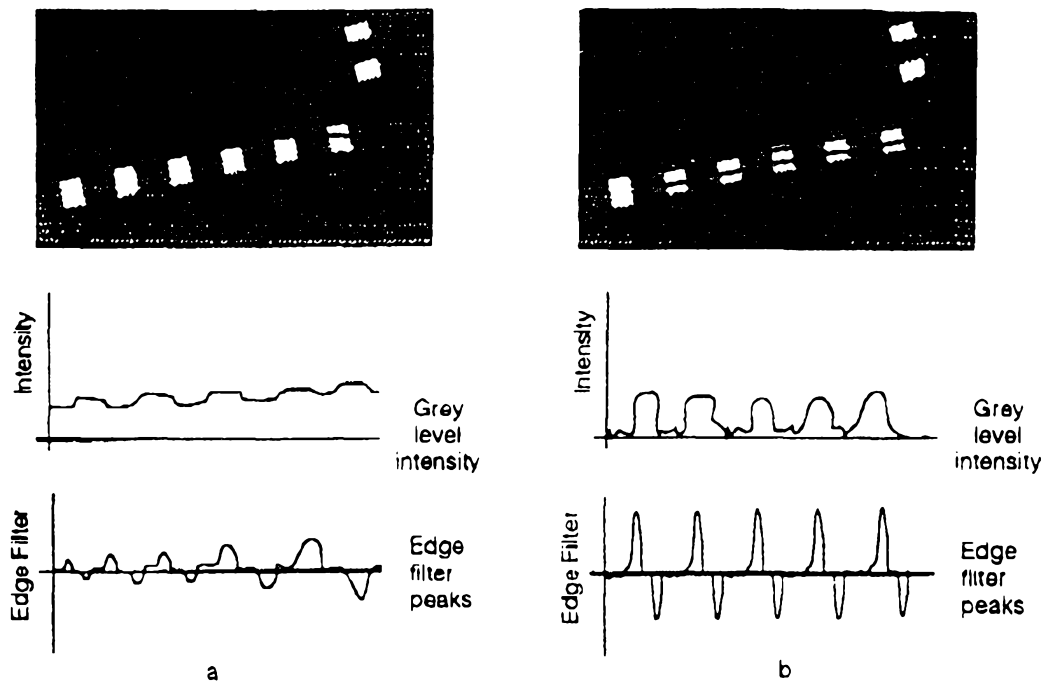
Figure 113. Skewed projection (a) and rotated projection (b)
