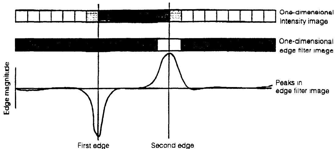
Figure 106. An edge filter is applied to the one-dimensional image that results from projection
