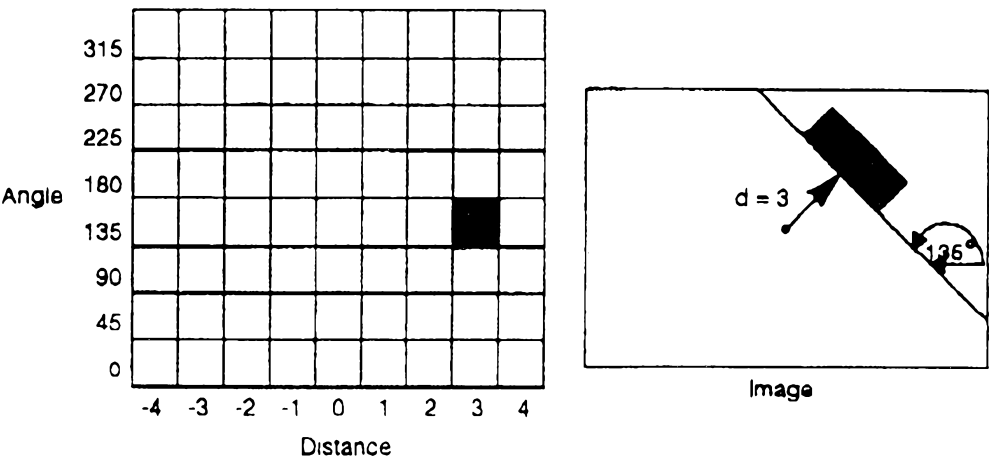
Figure 84. Hough space containing a single line
