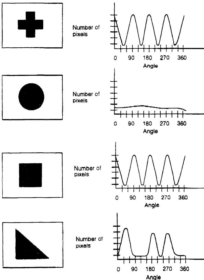
Figure 81. Assorted shapes with their angle histograms
