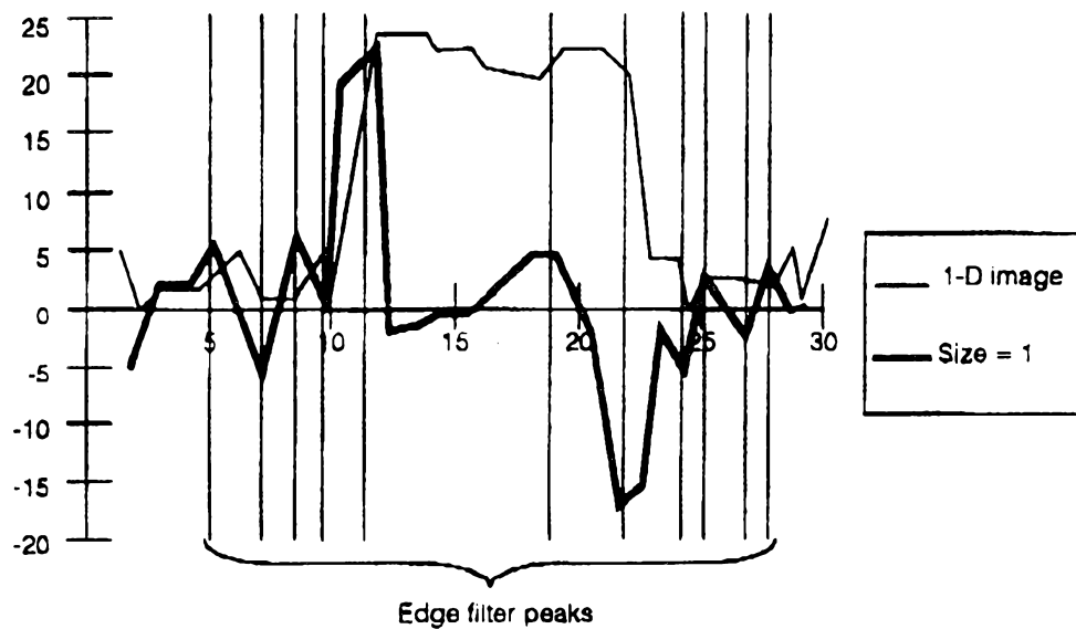
Figure 117. An edge filter size of 1 is typically too small.
