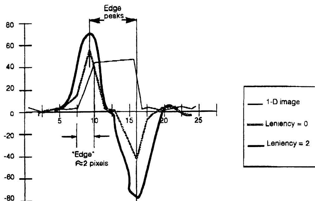
Figure 119. The effect of leniency on an edge filter image
