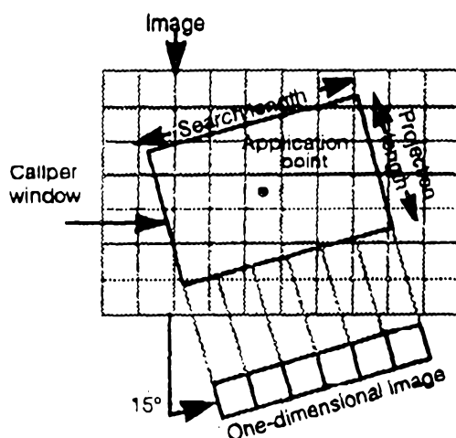
Figure 111. Rotated window projection
