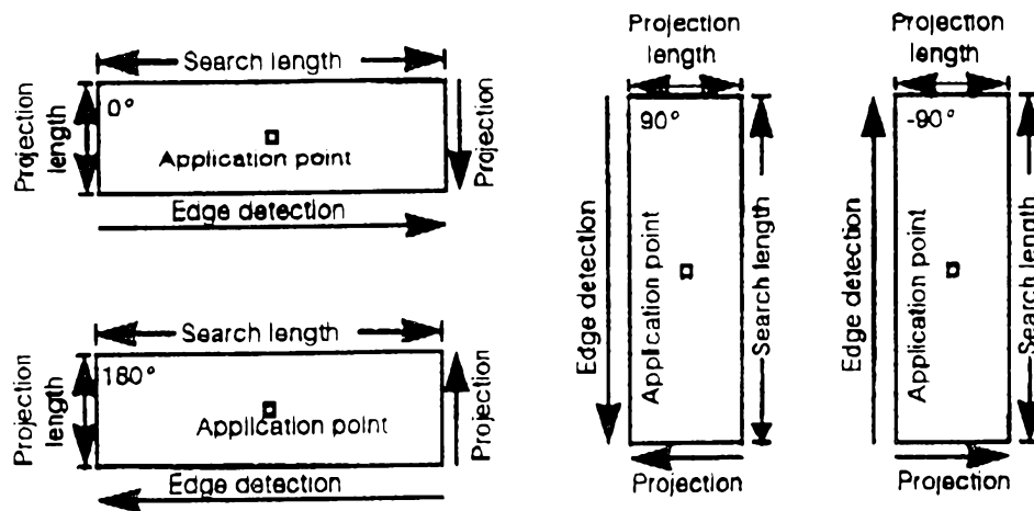
Figure 108. The caliper window at 90° rotations
