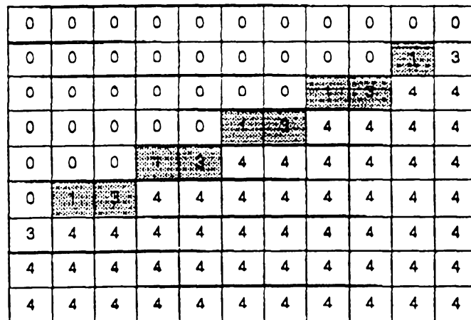
Figure 71. Highest magnitude edge pixels in an image
