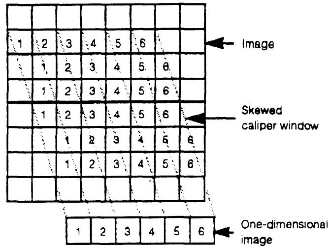
Figure 110. Skewed window projection without interpolation
