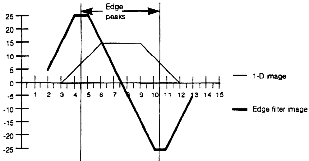
Figure 116. Edge filter image graph vs. one-dimensional image graph
