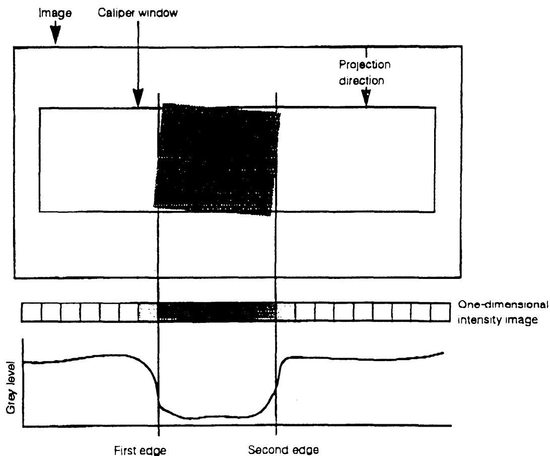
Figure 105. Overview of the Caliper Tool
