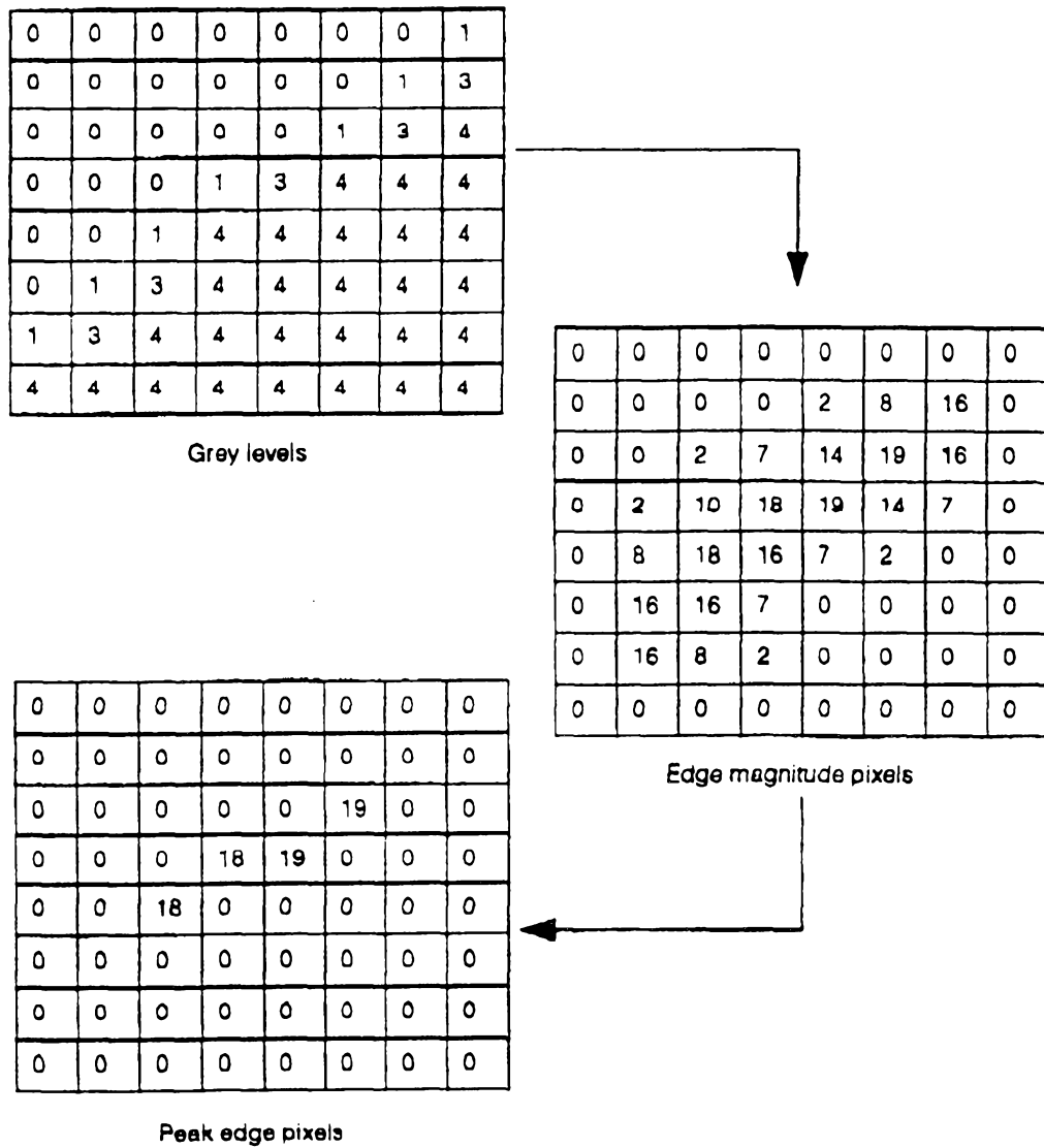
Figure 80. Peak detecting an edge magnitude image to determine actual edge
