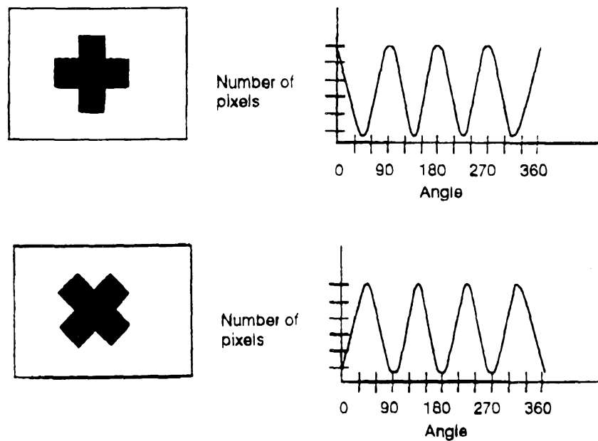
Figure 82. Effect of rotation on angle histogram
