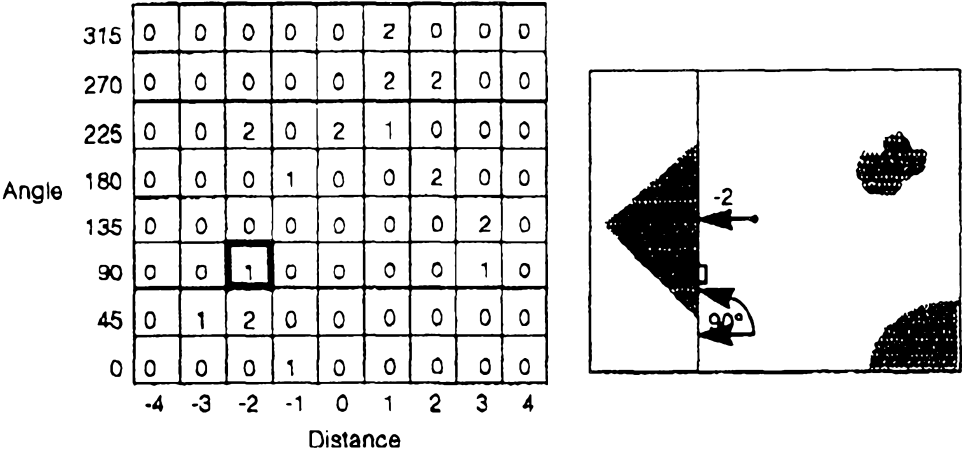
Figure 87. The bin in Hough space for the edge pixel's line is incremented.
