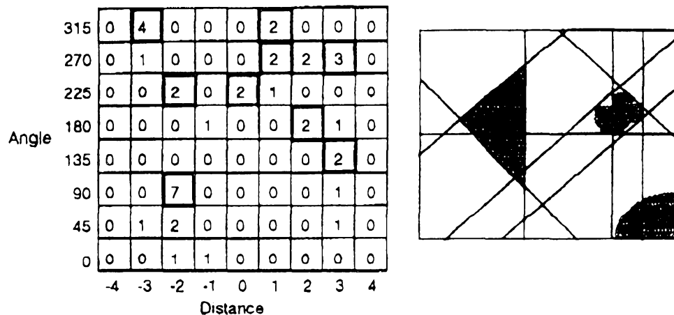
Figure 89. The peak-detected Hough space and the input image, with lines added
