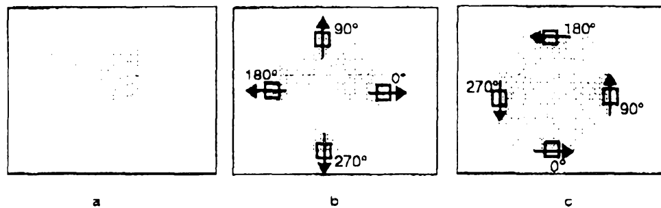
Figure 85. Four edges in an image (a), edge angles at four edge pixels (b), and line angles at those pixels (c)
