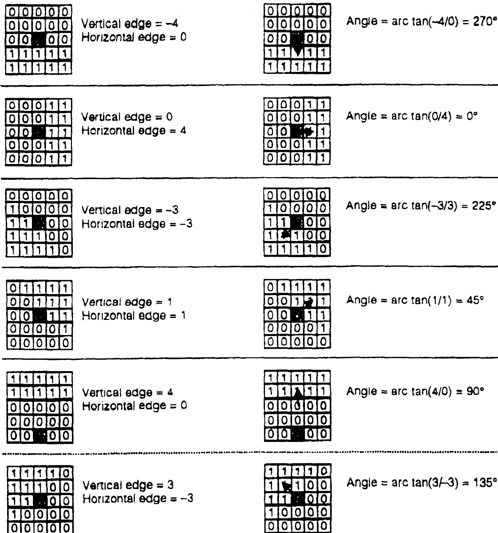
Figure 78. Computing the angle of various edges
