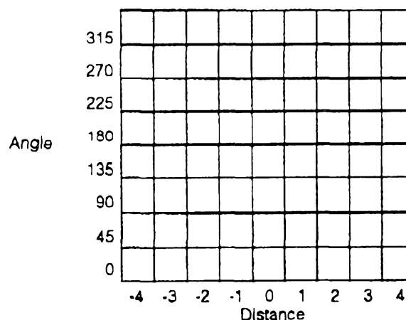
Figure 83. Hough space
