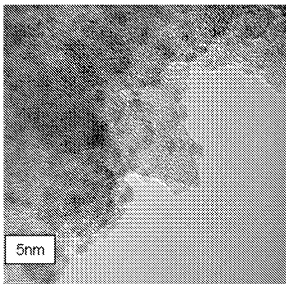
Figure 6: HRTEM images of Example 18 (trimeric Hf).
