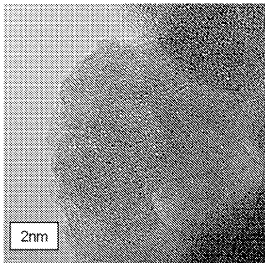
Figure 1: HRTEM images of Example 5 (monomeric Zr).
