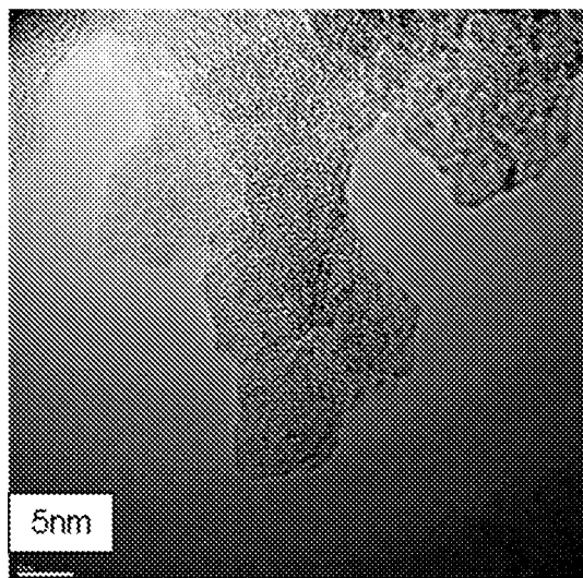
Figure 2: HRTEM images of Example 7 (monomeric Zr).
