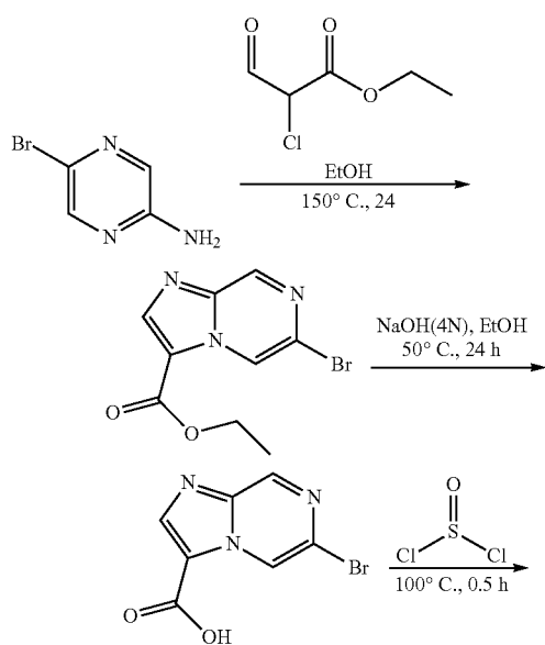
Reaction Scheme G:
