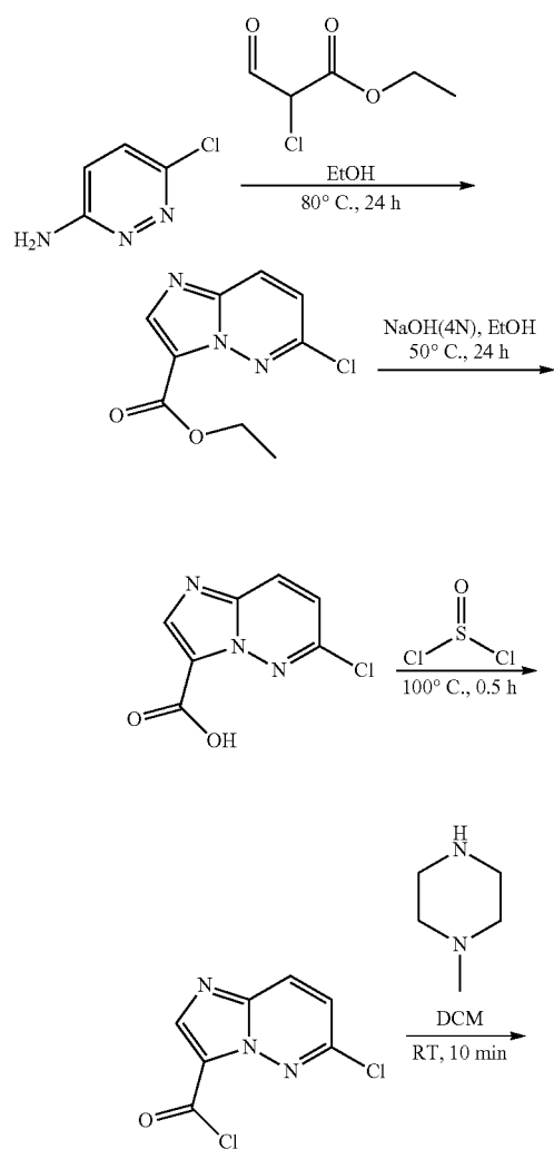
Reaction Scheme I
