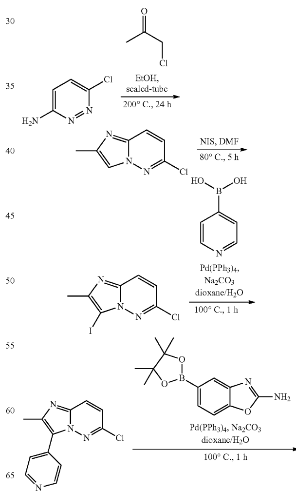
Reaction Scheme J
