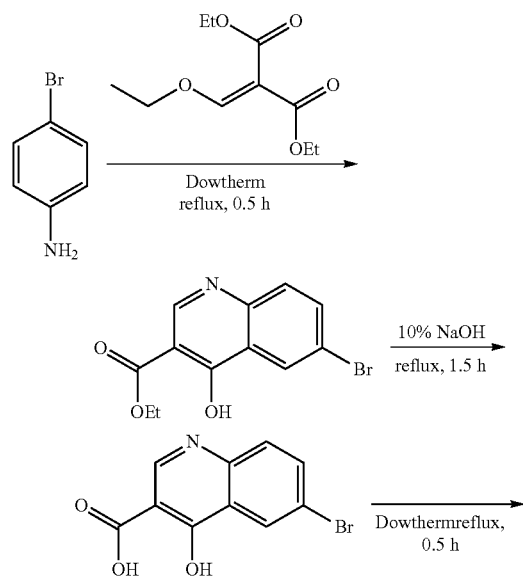
Reaction Scheme Y
