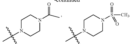
Subformula Ie
