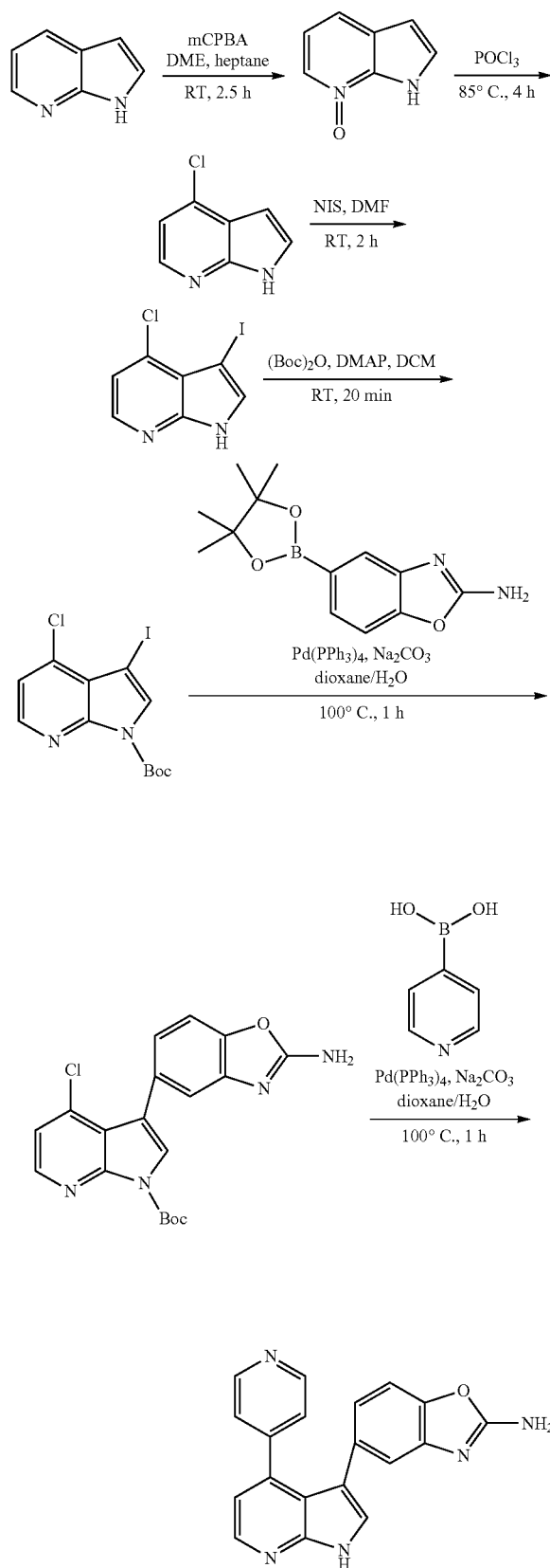
Reaction Scheme AD
