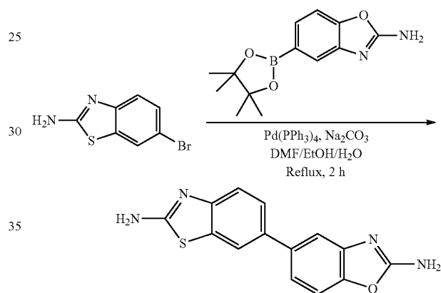
Reaction Scheme AF
