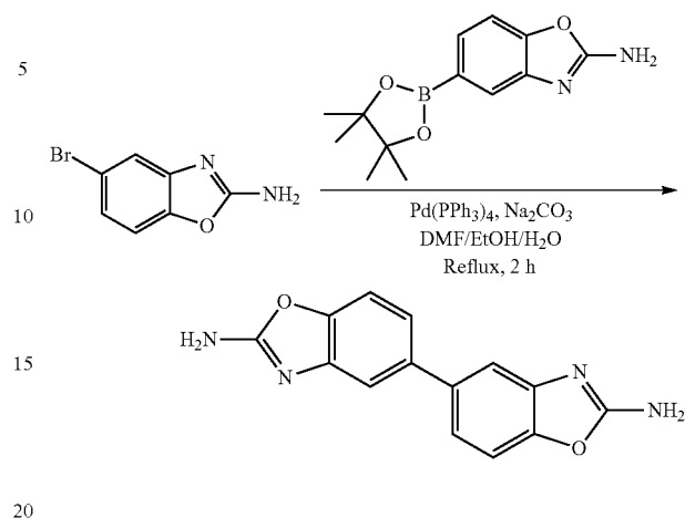
Reaction Scheme AE
