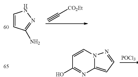
Reaction Scheme M:
