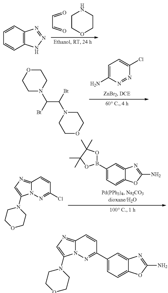
Reaction Scheme K
