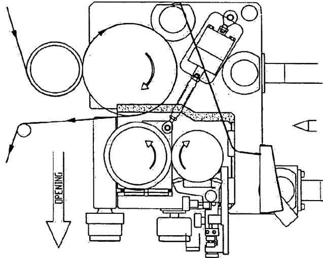
SEPARATION OF CONVEYOR/SPREADER ROLLER
