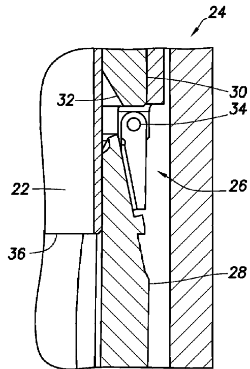
FIG. 2 (PRIOR ART)
