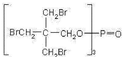
(Formula II)
