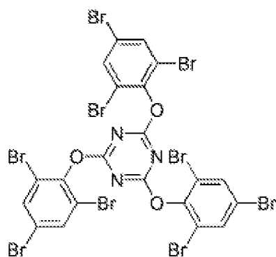
(Formula I)
