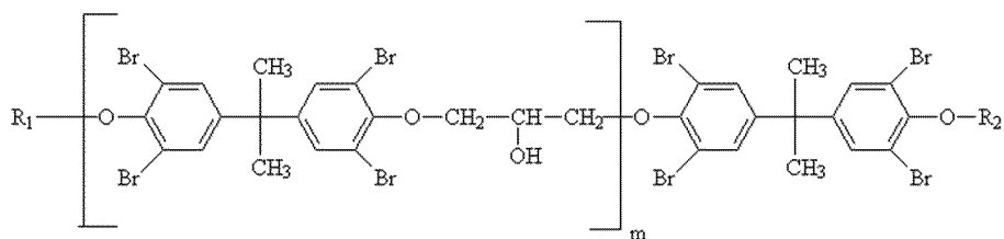
(Formula IV)
