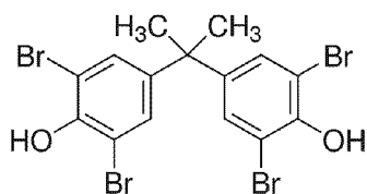
(Formula III)
