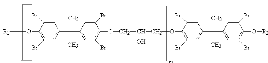
(Formula IV)
