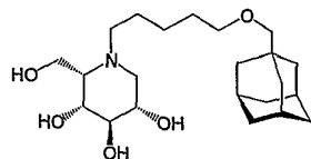
N -(adamantane-1-yl-methoxypentyl)-L-ido-deoxy-
