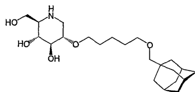
2- O -(adamantane-1-yl-methoxypentyl)-deoxy-
