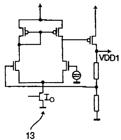
Fig. 5 PRIOR ART
