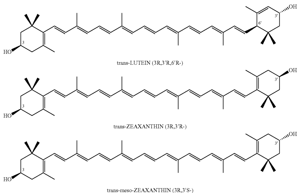
FIG. 1. Chemical structures of carotenoids
