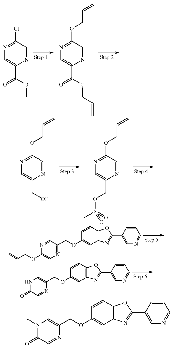
Step 1, Method 28: Prop-2-en-1-yl 5-(prop-2-en-1-yloxy)pyrazine-2-carboxylate
