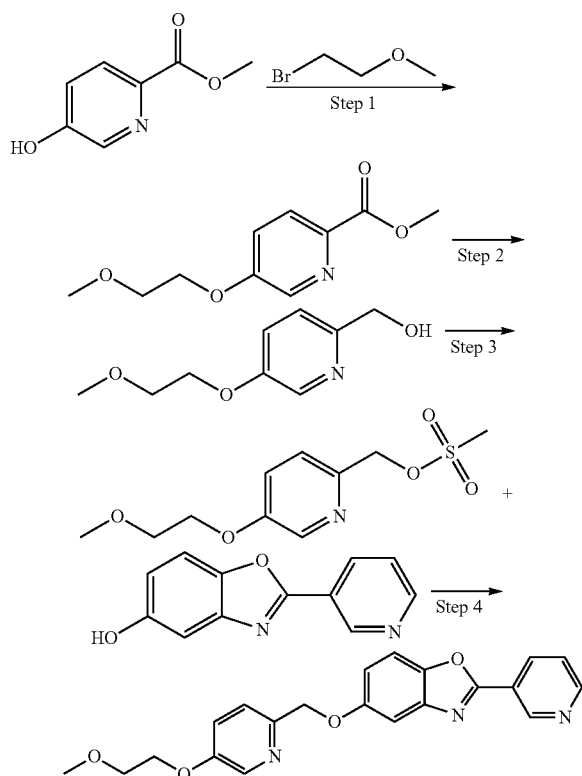
Step 1, Method 43: Methyl 5-(2-methoxyethoxy)pyridine-2-carboxylate
