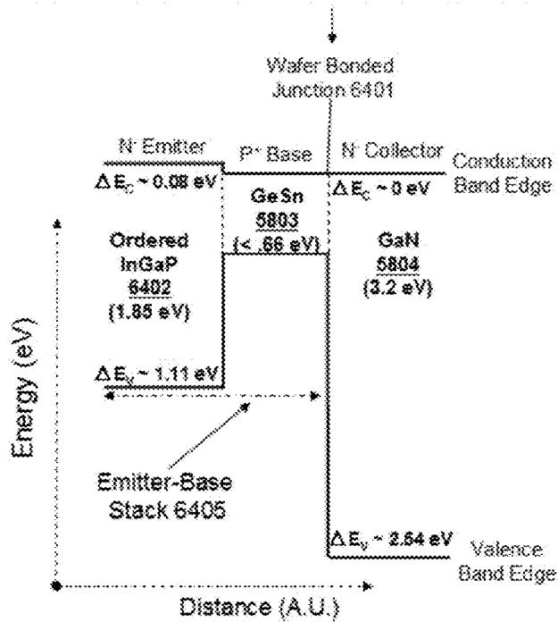
NPN InGaP Emitter – GeSn Base – GaN Collector Double HBT 6400
