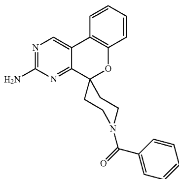
1'-(phenylcarbonyl)spiro[chromeno[3,4-d]pyrimidine-5,4'-piperidin]-3-amine
