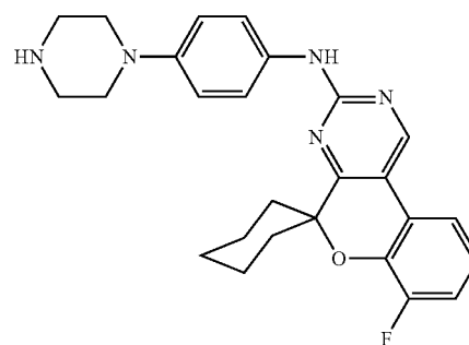
7-fluoro-N-(4-(1-piperazinyl)phenyl)spiro[chromeno[3,4-d]pyrimidine-5,1'-cyclohexan]-3-amine
