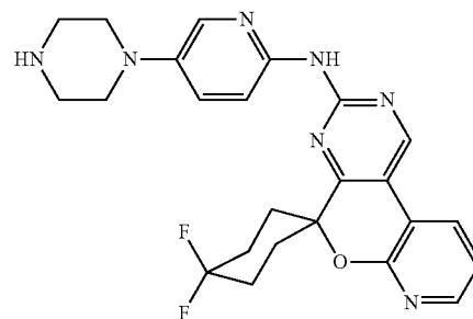
4,4-difluoro-N-(5-(1-piperazinyl)-2-pyridinyl)spiro[cyclohexane-1,5'-pyrido[3',3':5,6]pyrano[3,4-d]pyrimidin]-3'-amine
