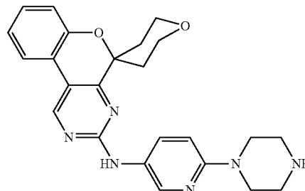
N-(6-(1-piperazinyl)-3-pyridinyl)-2',3',5',6'-tetrahydrospiro[chromeno[3,4-d]pyrimidine-5,4'-pyran]-3-amine
