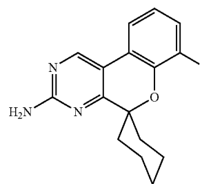
7-fluorospiro[chromeno[3,4-d]pyrimidine-5,1'-cyclohexan]-3-amine
