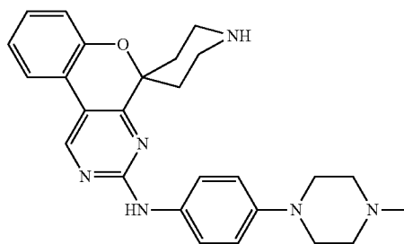
N-(4-(4-methyl-1-piperazinyl)phenyl)spiro[chromeno[3,4-d]pyrimidine-5,4'-piperidin]-3-amine
