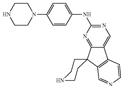
N-(4-(1-piperazinyl)phenyl)spiro[indeno[2,1-d]pyrimidine-9,4'-piperidin]-2-amine
