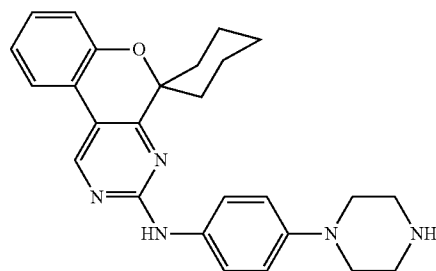
N-(4-(1-piperazinyl)phenyl)spiro[chromeno[3,4-d]pyrimidine-5,1'-cyclohexan]-3-amine
