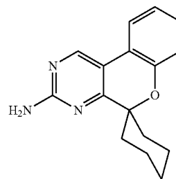
spiro[chromeno[3,4-d]pyrimidine-5,1'-cyclohexan]-3-amine
