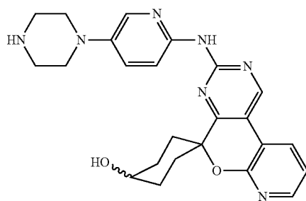
3'-β5-(1-piperazinyl)-2-pyridinylamino)spiro[cyclohexane-1,5'-pyrido[3',2':5,6]pyrano[3,4-d]pyrimidin]-4-ol
