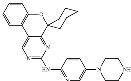
N-(5-(1-piperazinyl)-2-pyridinyl)spiro[chromeno[3,4-d]pyrimidine-5,1'-cyclohexan]-3-amine
