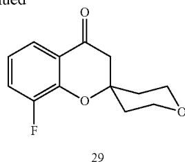
8-Fluoro-2',3',5',6'-tetrahydrospiro[chromene-2,4'-pyran]-4(3H)-one (29)
