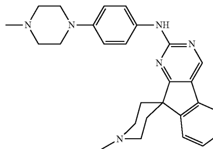
1'-methyl-N-(4-(4-methyl-1-piperazinyl)phenyl)spiro[indeno[2,1-d]pyrimidine-9,4'-piperidin]-2-amine
