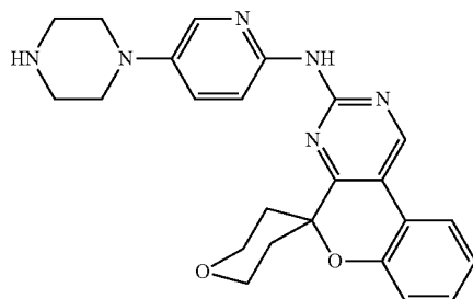
N-(5-(1-piperazinyl)-2-pyridinyl)-2',3',5',6'-tetrahydrospiro[chromeno[3,4-d]pyrimidine-5,4'-pyran]-3-amine
