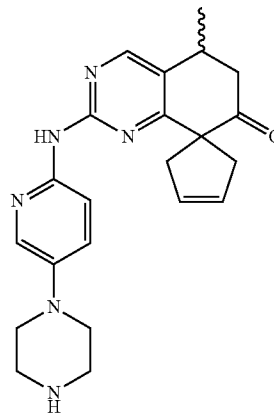
(5'R)-5'-methyl-2'-((5-(1-piperazinyl)-2-pyridinyl)amino)-5',6'-dihydro-7'H-spiro[cyclopent-3-ene-1,8'-quinazolin]-7'-one
