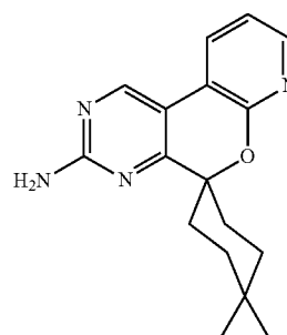
4,4-dimethylspiro[cyclohexane-1,5'-pyrido[3',3':5,6]pyrano[3,4-d]pyrimidin]-3'-amine
