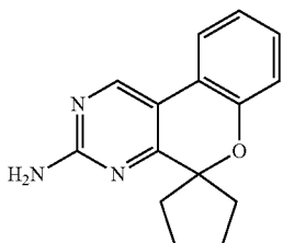
spiro[chromeno[3,4-d]pyrimidine-5,1'-cyclopentan]-3-amine
