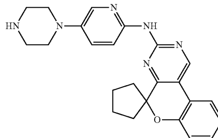
N-(5-(1-piperazinyl)-2-pyridinyl)spiro[chromeno[3,4-d]pyrimidine-5,1'-cyclopentan]-3-amine
