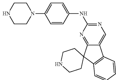
N-(4-(1-piperidinyl)phenyl)spiro[indeno[2,1-d]pyrimidine-9,4'-piperidin]-2-amine
