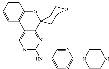
N-(2-(1-piperazinyl)-5-pyrimidinyl)-2',3',5',6'-tetrahydrospiro[chromeno[3,4-d]pyrimidine-5,4'-pyran]-3-amine
