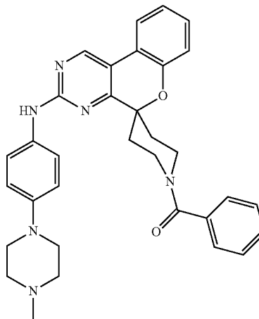
N-(4-(4-methyl-1-piperazinyl)phenyl)-1'-(phenylcarbonyl)spiro[chromeno[3,4-d]pyrimidine-5,4'-piperidin]-3-amine
