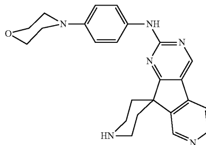
N-(4-(4-morpholinyl)phenyl)spiro[indeno[2,1-d]pyrimidine-9,4'-piperidin]-2-amine
