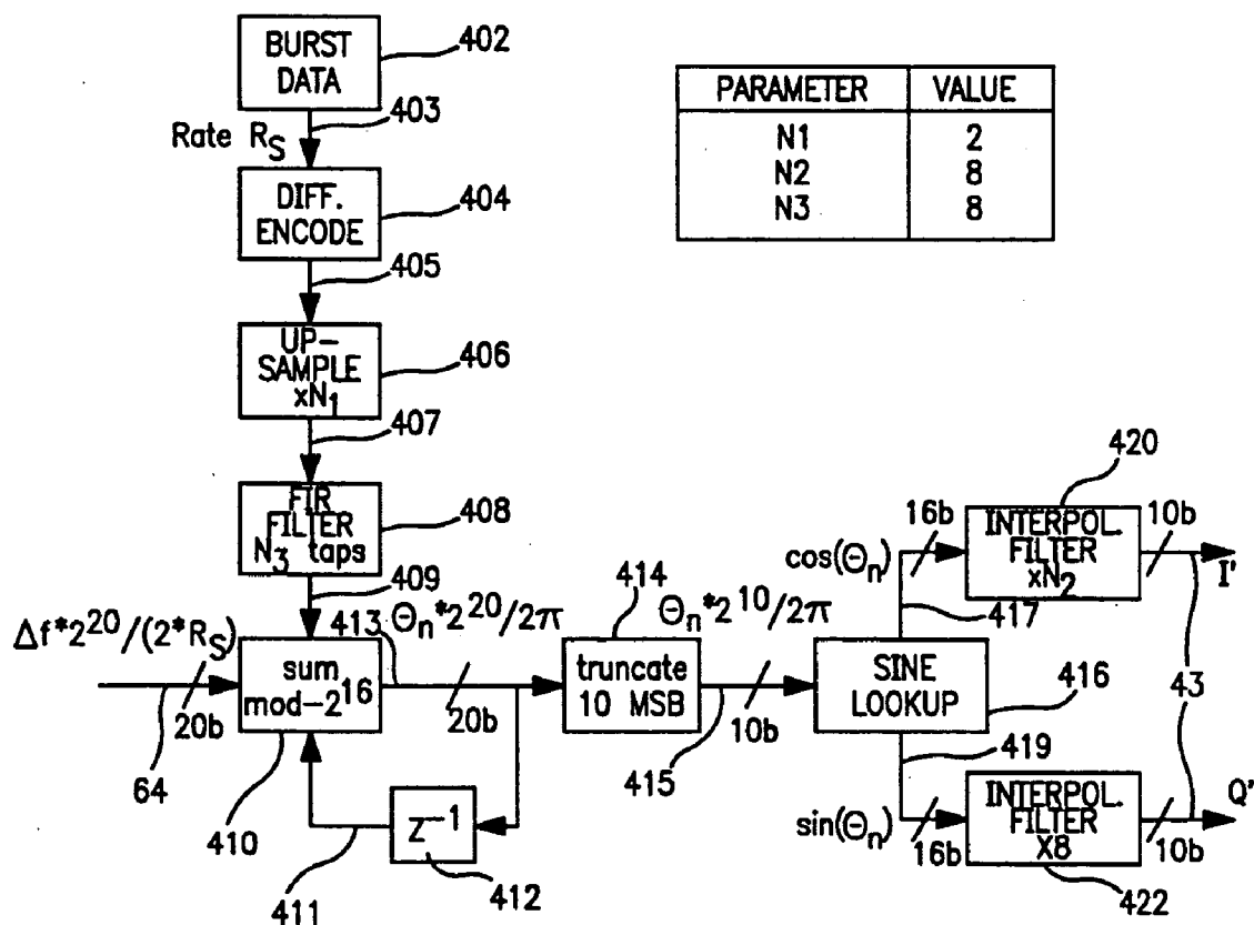
CONTINUOUS PHASE MODULATOR AND UPLINK PHASE ROTATOR
