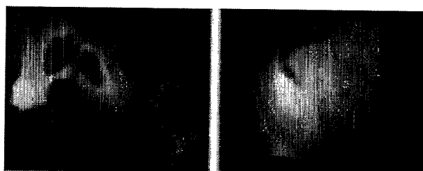
GFP-NES1
