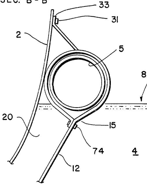
FIG. 6 SEC. B - B'
