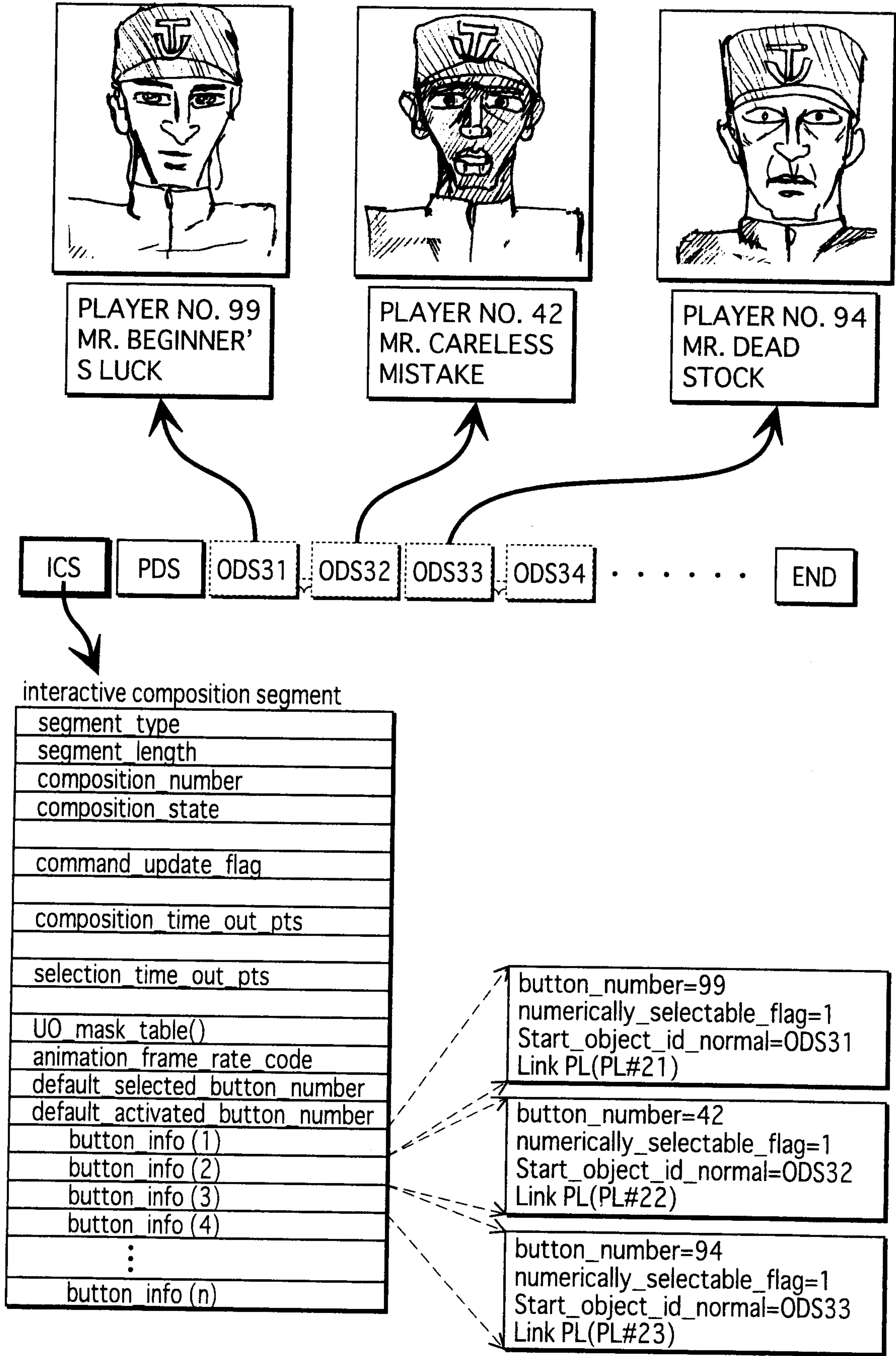
FIG.18 PLAYERS LIST
