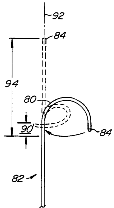
FIG. 5. PRIOR ART
