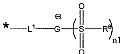
General Formula (A3-1)
