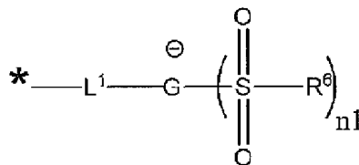
General Formula (A3-1)
