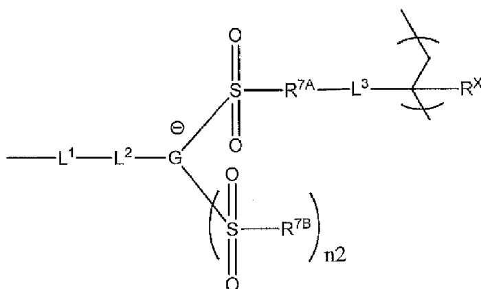
General Formula (A4-3-1)
