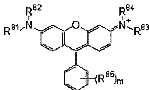
General Formula (J)
