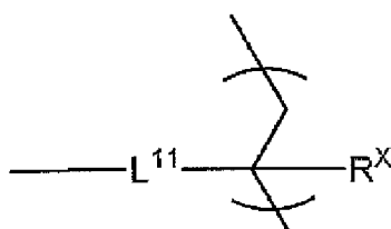
General Formula (A4-1-2)
