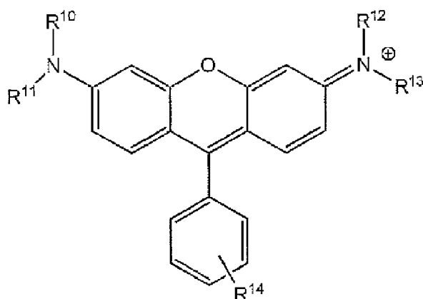
General Formula (A4-1)
