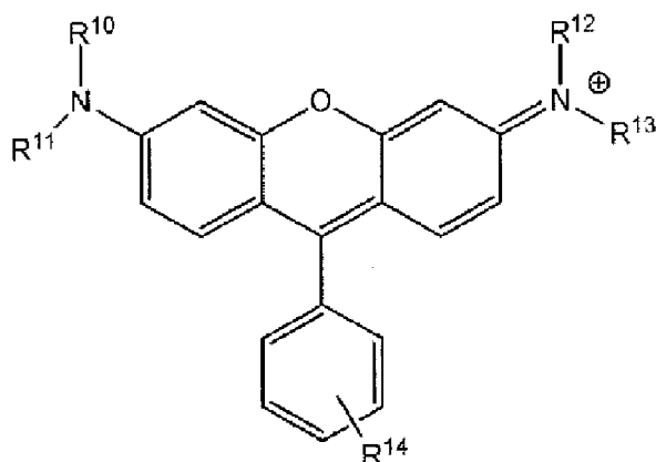
General Formula (A4-3)
