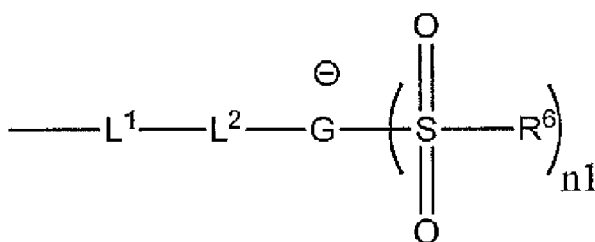
General Formula (A4-1-1)
