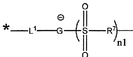
General Formula (A3-2)
