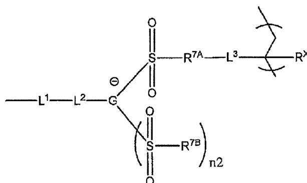
General Formula (A4-3-1)
