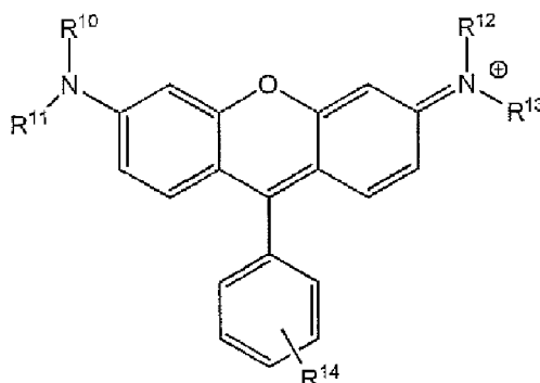
General Formula (A4-1)
