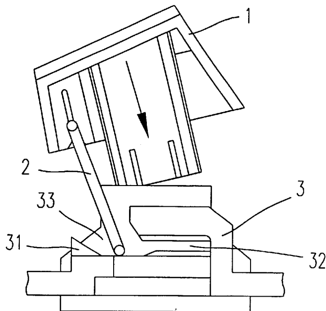
Fig. 1(b)(PRIOR ART)
