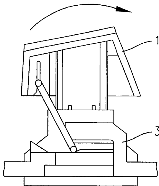
Fig. 1(d)(PRIOR ART)
