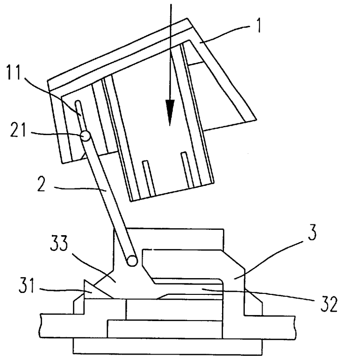
Fig. 1(a)(PRIOR ART)
