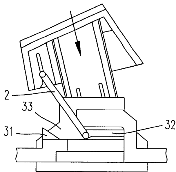
Fig. 1(c)(PRIOR ART)
